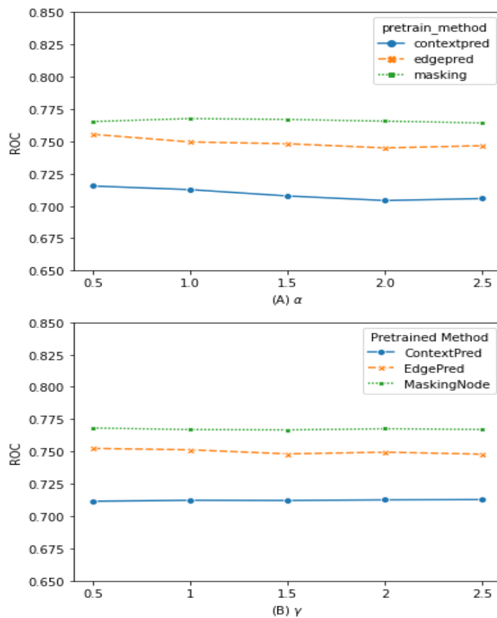
Figure 9. Hyper-parameters Sensitivity.
