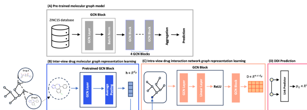
Figure 2. The schematic diagram of our SMG-DDI model.
