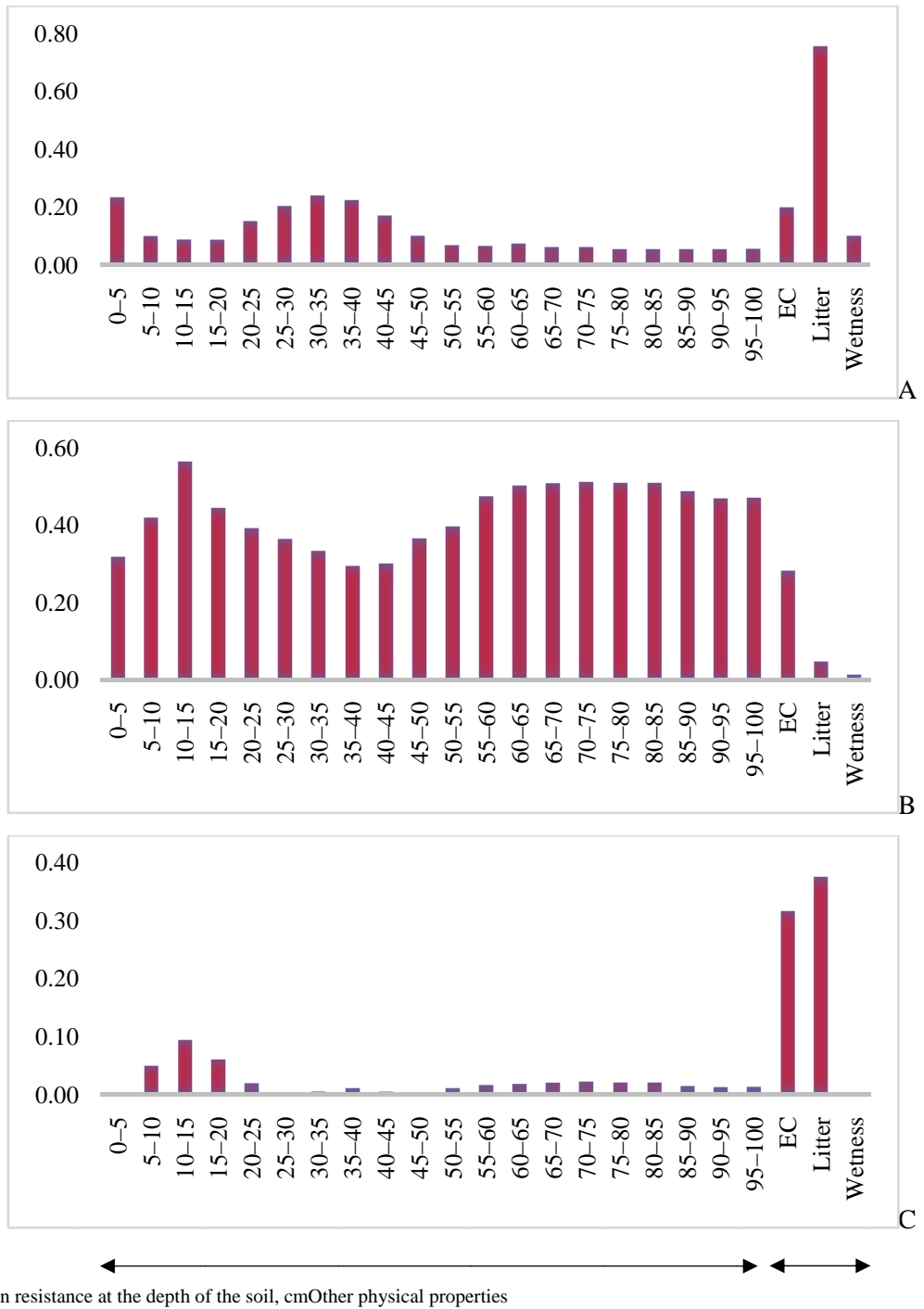
Fig. S1. Decrease in the variance of soil physical properties explained by year, polygon, and reconstruction when accounting for the influence of predictors as partial variables: A – year as a partial variable; B – polygons as a partial variable; C – reconstruction as a partial variable
