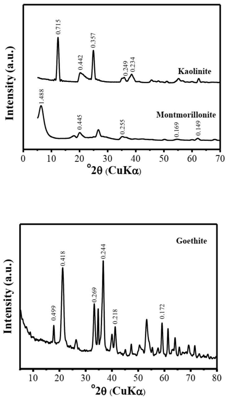
Fig. S1. Powder XRD patterns of kaolinite, montmorillonite and goethite
