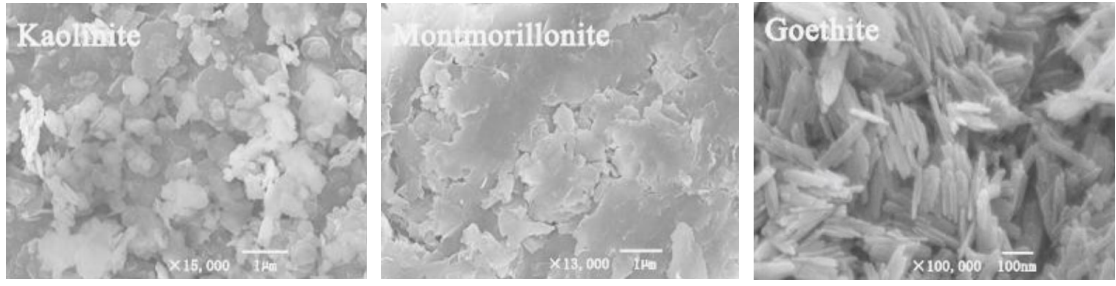
Fig. S2. Scanning electron microscope (SEM) images for minerals
