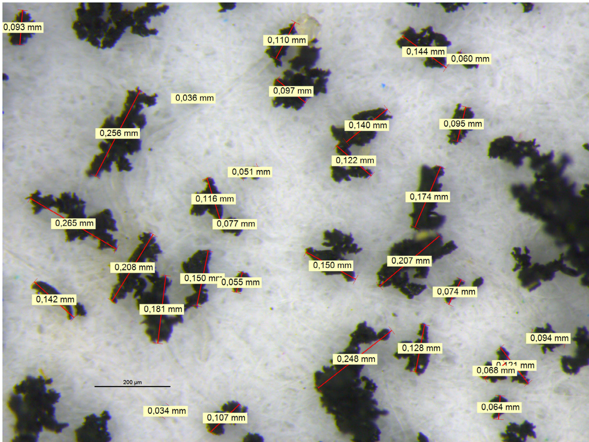
Fig. S1: photographic processing of tire particle size to determine average diameter and size range. Always the longest length of the particle was chosen.
