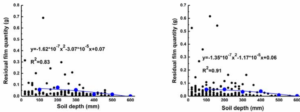
Fig. S2. The weight distribution of film debris in soils with different mulching times
