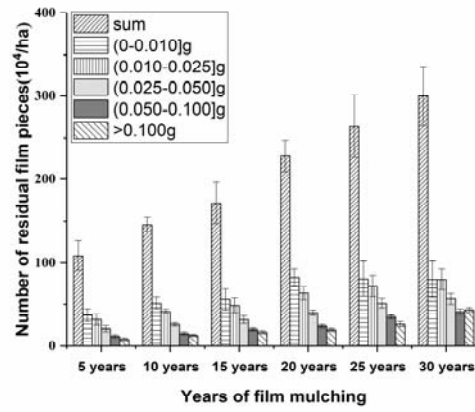
Fig. S2. The weight distribution of film debris in soils with different mulching times
