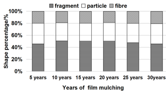
Fig. S4. The distribution of different shape MPs with varying mulching times.
