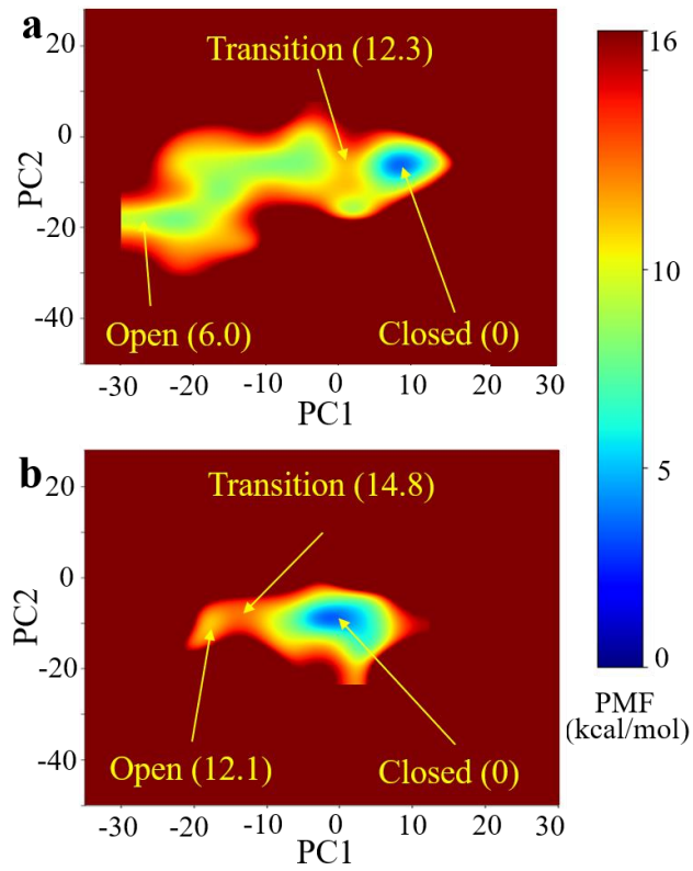
Figure S1: Two-dimensional free energy profiles on the principal components (PC1 and PC2) in (a) one aMD simulation of the apo YTH, and (b) one aMD simulation of the YTH-A3 RNA.
