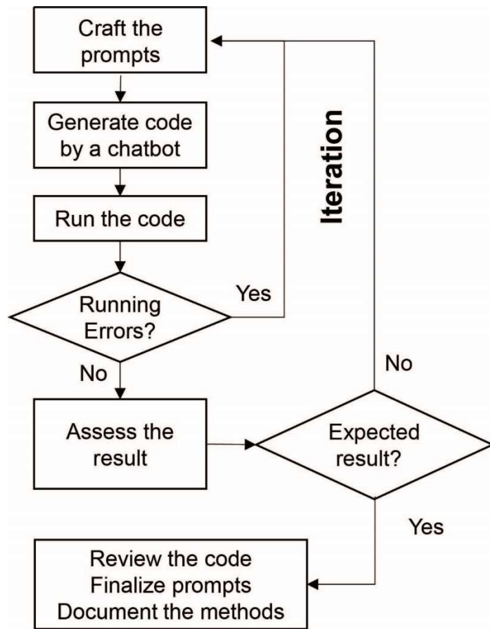
Figure S1: The OPTIMAL model for LLM chatbot-assisted scientific data analysis
