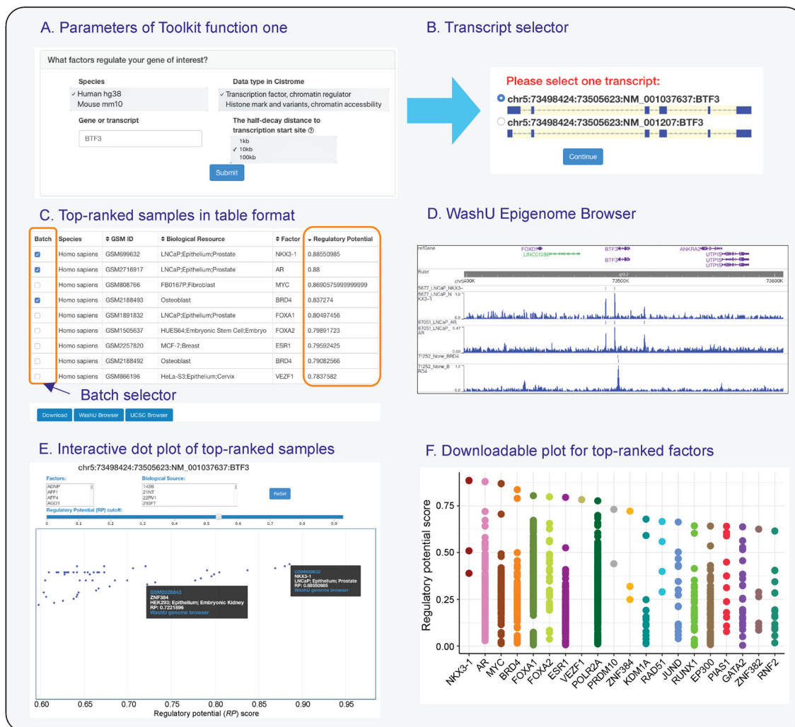
Figure 2. Introduction to the first function of Cistrome DB Toolkit, “what factors regulate your gene of interest?” (A) An input box for gene name or RefSeq transcript ID, and parameter selections for species of human (hg38) and mouse (mm10), data type of “transcription factors, chromatin regulator” and “Histone mark and variants, chromatin accessibility”, and half decay rate of 1 kb, 10 kb, and 100 kb to weight peaks up- and down-stream of TSS. (B) Transcript selection only when a gene symbol matches multiple transcripts. (C) Results of top-ranked samples by the regulatory potential score. Select samples in the batch selector and click the bottom button to view tracks in Wash U or UCSC Browser. (D) A track example in the Wash U Epigenome Browser. (E) An interactive dot plot for showing ChIP-seq samples that RP score of the user-given gene greater than zero. Users filter samples by selecting factor or biological resources or moving the RP cutoff slider above the plot. ( F) A downloadable plot for showing 20 regulators with the highest score.
