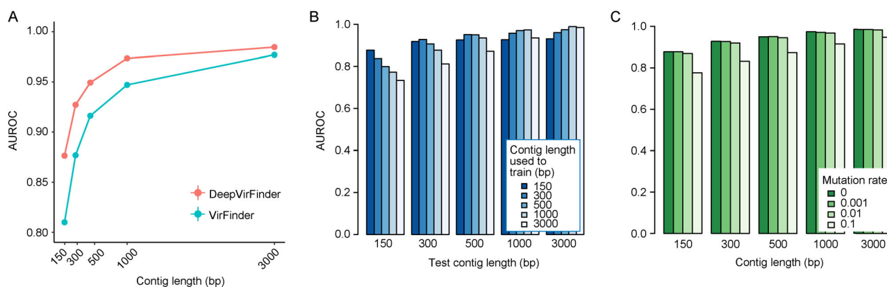
Figure 2. Comparison of DeepVirFinder with VirFinder and the effect of contig length and mutation rates on the performance of DeepVirFinder. (A) AUROCs for VirFinder and DeepVirFinder when trained on sequences before May 2015, and tested on sequences after May 2015. See Supplementary Fig. S1 for the exact numbers and the standard errors. (B) AUROCs for different combinations of sequence lengths used for training and testing. (C) AUROCs for prediction when adding mutations at different rates.
