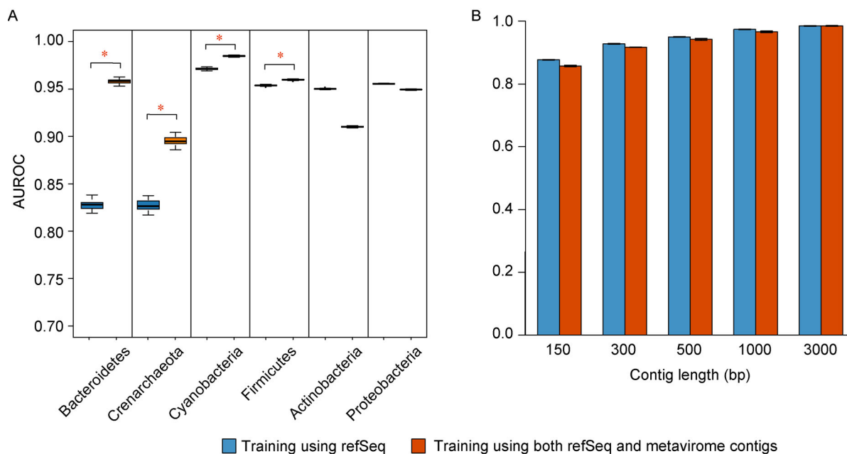
Figure 3. Comparison of AUROCs between the model trained using only viral RefSeq, and the model trained using the enlarged dataset including millions of sequences from metavirome. (A) The AUROCs for predicting 500 bp viral sequences from different host phyla. The under-represented viruses groups, viruses infecting Crenarchaeota, Bacteroidetes (B) the overall AUROCs between the two models at different sequence lengths.
