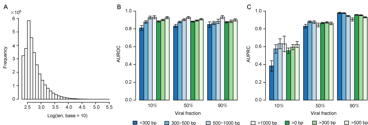
Figure 4. Evaluation of the performance of DeepVirFinder on viral contigs of variable lengths in simulated metagenomic samples with various viral fractions. (A) The distribution of contig length used for simulating metagenomic samples, and the (B) AUROC and (C) AUPRC for predicting viral sequences with various viral fractions (10%, 50% and 90%) for contigs of different lengths.
