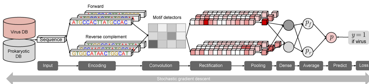
Figure 1. The deep learning framework of DeepVirFinder. Sequences from viral genomes and prokaryotic genomes are used for training the model. The neural network is composed by a convolutional layer, a max pooling layer, a dense layer with ReLU activation function, and a final dense layer with sigmoid function to generate the prediction score between 0 and 1. The higher score indicates the more likely a sequence is from viral genomes. For each sequence, both forward and its reverse complementary are fed into the same neural networks, and the final prediction score is the average of the two corresponding prediction scores.
