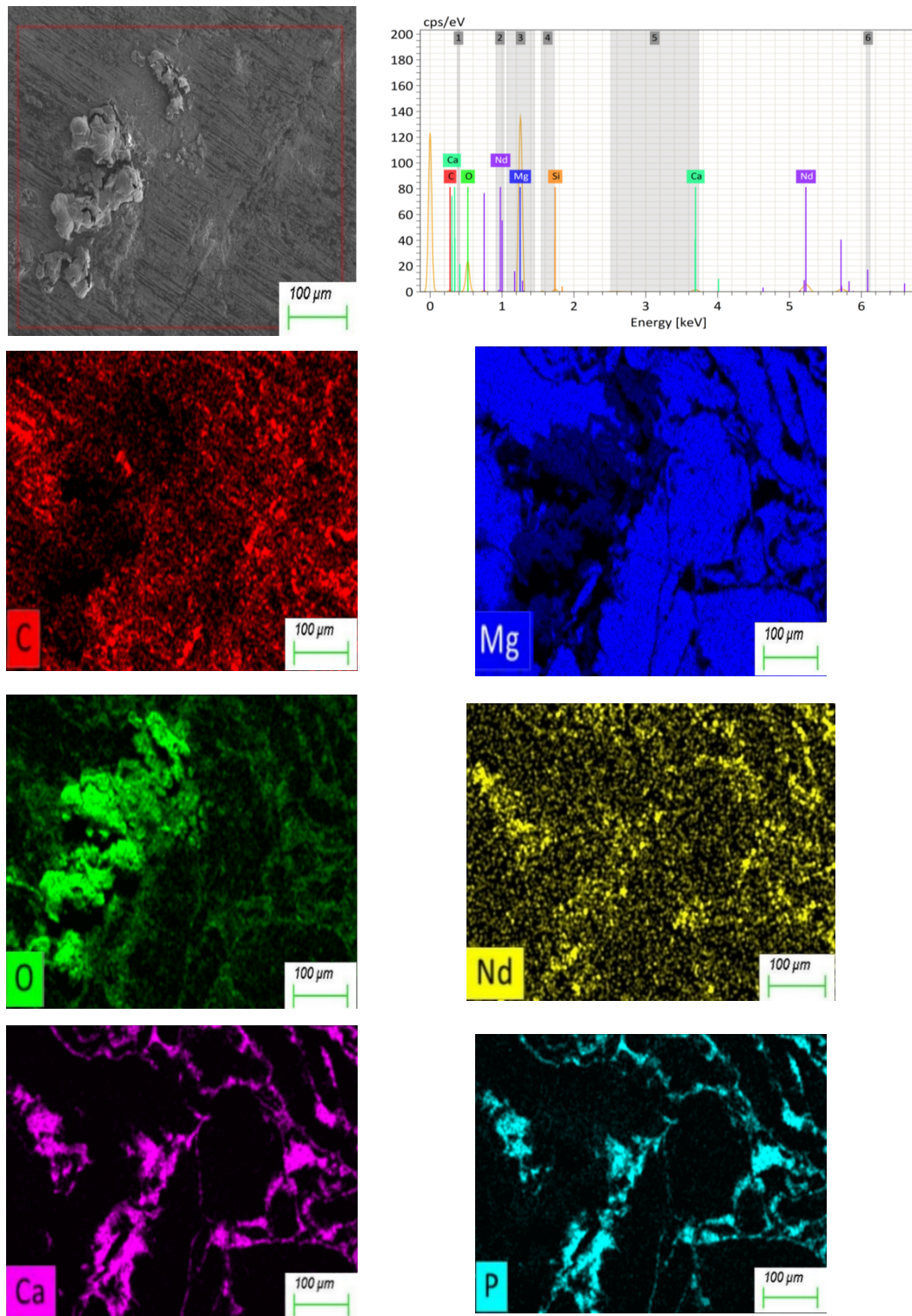
Figure 9. EDS spectra and elemental mapping of Mg-HA-1Nd 2 O 3 composite samples at 10 N load.
