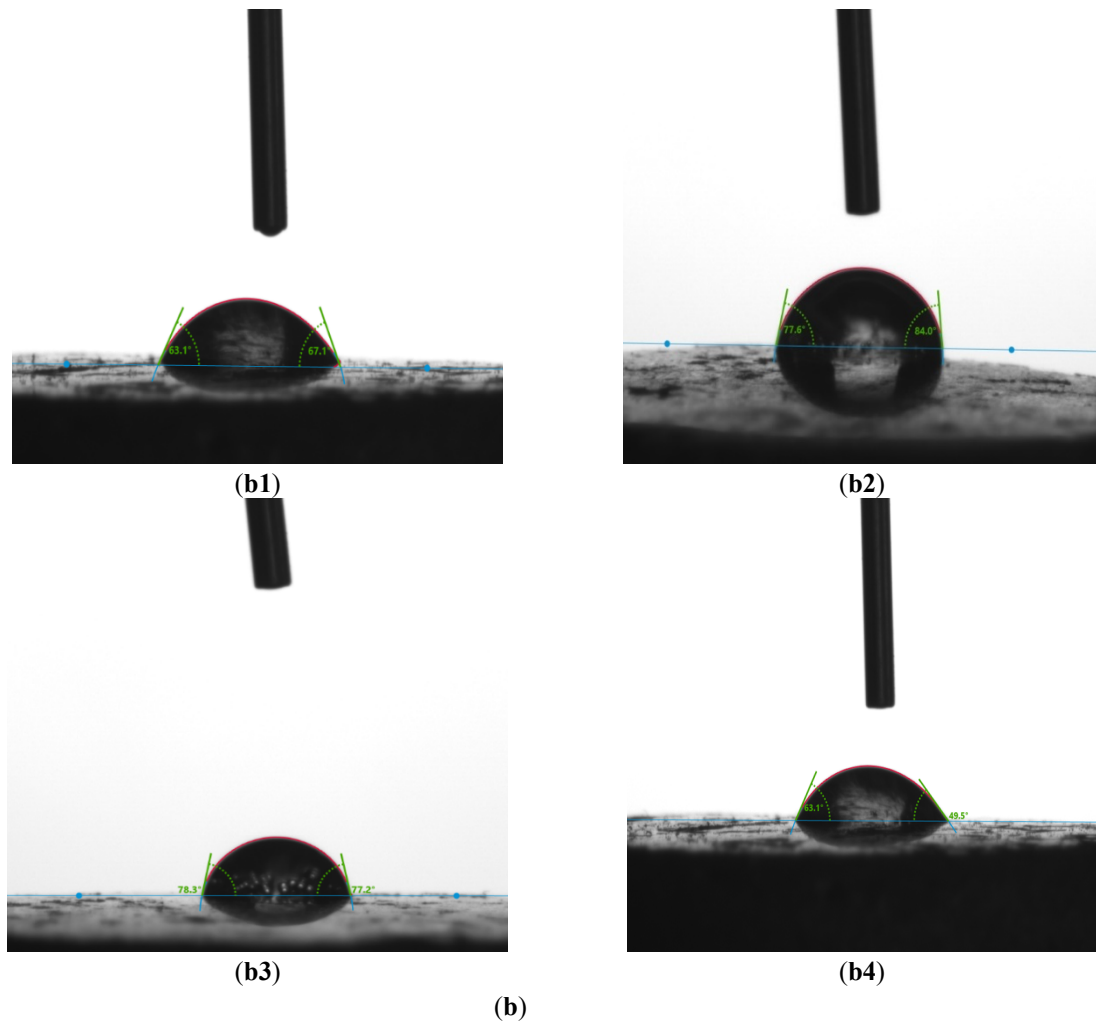
Figure 12. (a): Contact angle measurements of composite samples using sessile drop analyzer. (b) Schematic configuration of sessile drop contact angle measurements for (b1) Mg-HA-1Nd 2 O 3 (b2) Mg-HA-1.5Nd 2 O 3 (b3) Mg-HA-2Nd 2 O 3 (b4) Mg-HA composite.
