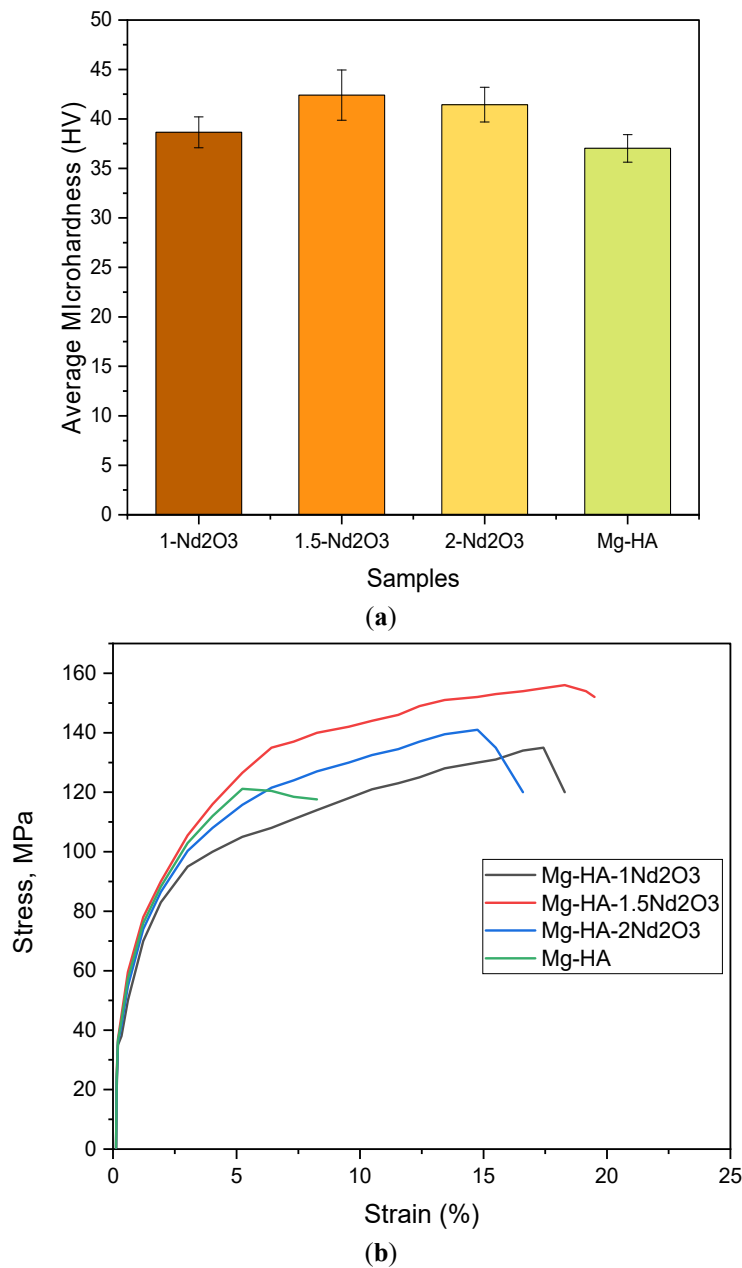
Figure 6. (a): Microhardness plot of composite samples showing effect of rare earth oxide %age vs. pure Mg-HA sample. (b): Tensile stress-strain curves of Mg-HA-xNd 2 O 3 (x = 1%, 1.5%, and 2%) composite samples.
