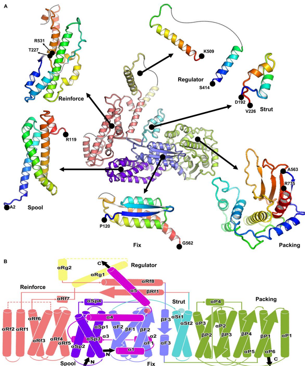
Fig. S9. Overall structure and topology diagram of pUL28. (A) Ribbon diagram of pUL28. The central image shows pUL28 colored as in Fig. 3a. Rainbow ribbon
