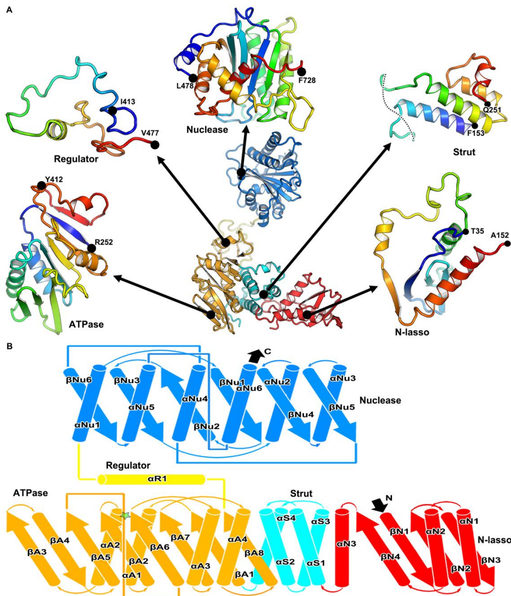
Fig. S5. Overall structure and topology diagram of pUL15. (A) Overall structure
