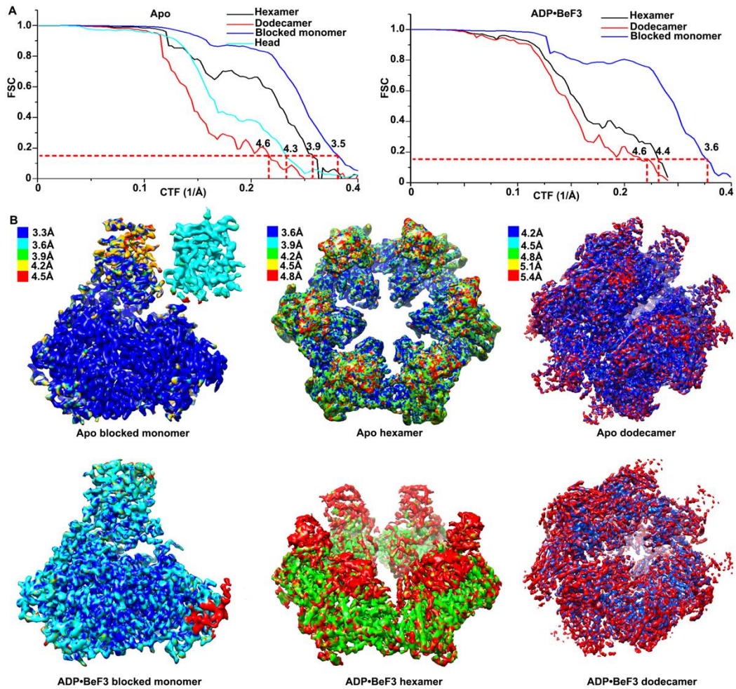
Fig. S2. Resolution evaluation of the cryoEM maps. (A) The gold-standard FSC curves. FSC plots of the apo terminase assembly (left) including the hexamer, dodecamer, blocked monomer and head region, the ADP•BeF3-bound terminase assembly (right) containing the hexamer, dodecamer and blocked monomer based on the FSC=0.143 criterion are shown. (B) The local resolution was evaluated by ResMap ((Kucukelbir et al. , 2014)).
