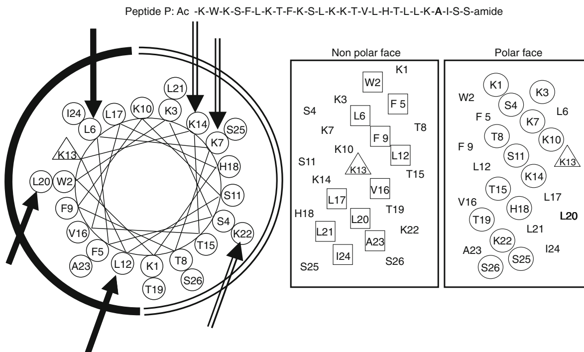
Figure 1. Representation of the parent peptide A12L/A20L as helical nets showing the polar/hydrophilic face (circled residues) and non-polar/hydrophobic face (boxed residues) and helical wheel, the lysine residue at position 13 of the sequence is denoted by a triangle. In the helical nets, the D-amino acid substitution sites are shown in bold and italic , while in the helical wheel, three single substitution sites are shown with solid arrows on the non-polar face as a solid arc and hollow arrows on the polar face as an open arc , respectively, Ac denotes N α -acetyl, and amide denotes C α -amide. One-letter codes are used for the amino acid residues.
