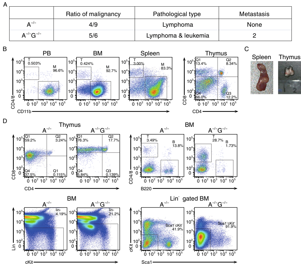
Figure 5. Gadd45a prevents the incidence of hematopoietic malignancies in ATM^{-/-} mice. (A) The ratio of malignancy, pathological type, and metastasis in ATM^{-/-} and ATM^{-/-} Gadd45a ^{-/-} mice are shown. (B–C) AML with spleen infiltration was observed in one ATM^{-/-} Gadd45a ^{-/-} mice (without lymphoma). The FACS plots in the indicated tissues and the pictures of spleen (infiltrated) and thymus (without lymphoma) of the AML mice are shown. (D) Representative FACS plots in the indicated tissues in ATM^{-/-} (lymphoma without BM infiltration) and ATM^{-/-} Gadd45a ^{-/-} (lymphoma with BM infiltration) mice with are shown.
