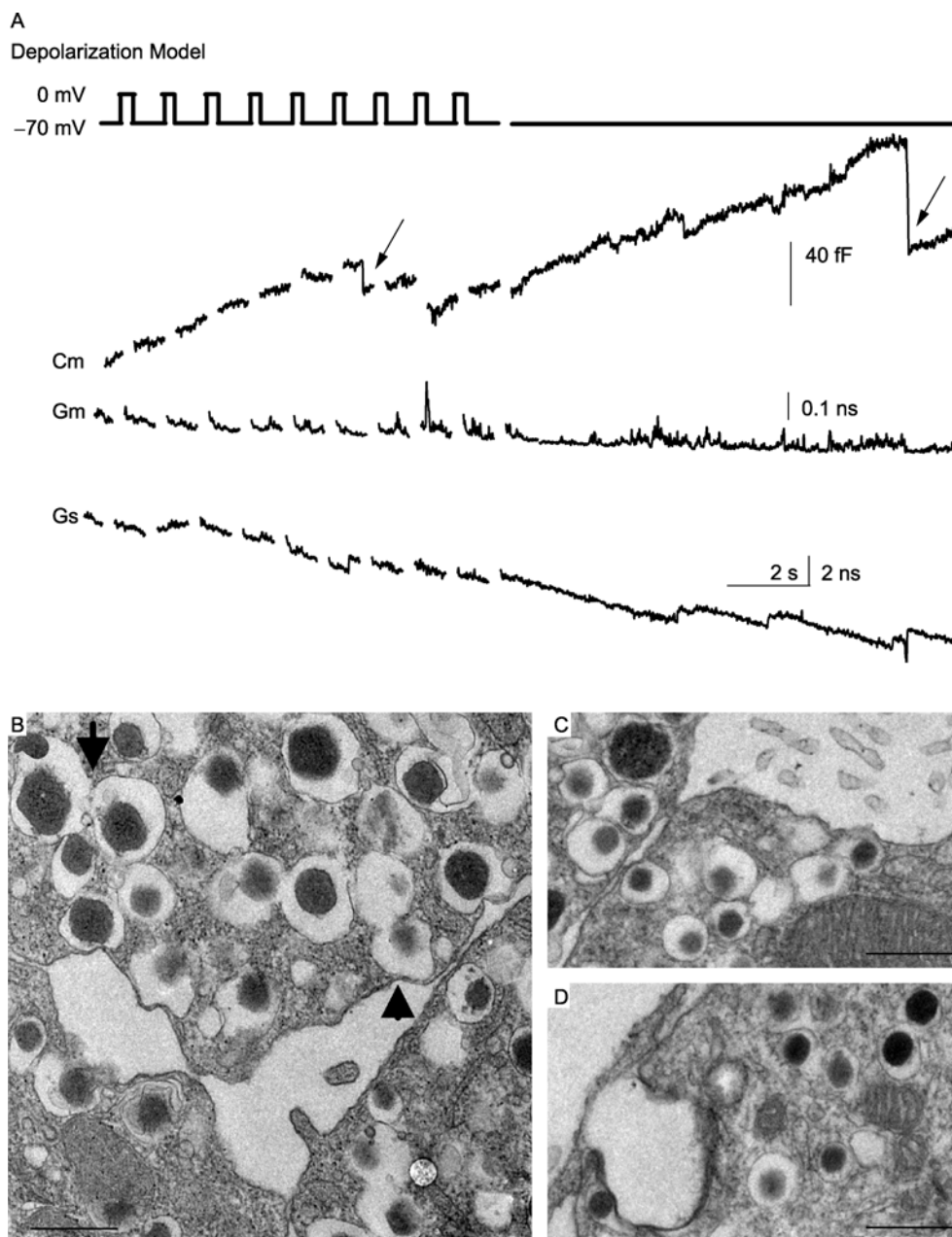
Figure 2. Depolarization elicit bulk-like endocytosis in pancreatic \beta cells. (A) Trains of ten 200-ms pulses (frequency 1 Hz) induced a capacitance jump ( C_m ), except for abrupt bulk endocytosis (arrows). The measured values of G_m and G_s are shown below the figure. (B) After 5 min of 20 mmol/L glucose stimulation, two insulin granules are contacted and fused with each other (indicated by arrow) and three fused granules are retrieval together after the release of the contents (indicated by arrow head). (C) Secretory granules fuse together (also partially emptied) after 70 mmol/L KCl stimulation for 5 min. (D) Large invagination connected to the plasma membrane after 70 mmol/L KCl stimulation. Scale bar: 500nm in all EM figures.
