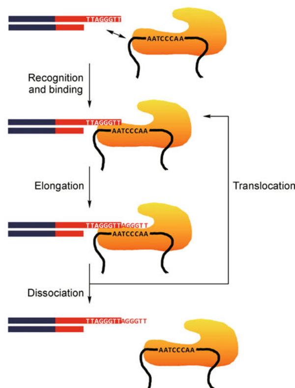
Figure 2. The telomerase reaction cycle. The telomerase reaction cycle consists of three distinct steps: substrate recognition and binding, where telomerase localises to the very 3' terminus of the G-rich overhang; elongation, where telomeric repeats are added by TERT using TERC as a template; and dissociation or translocation, where telomerase moves to the new 3' end of the chromosome to add another repeat, or releases the telomere.
