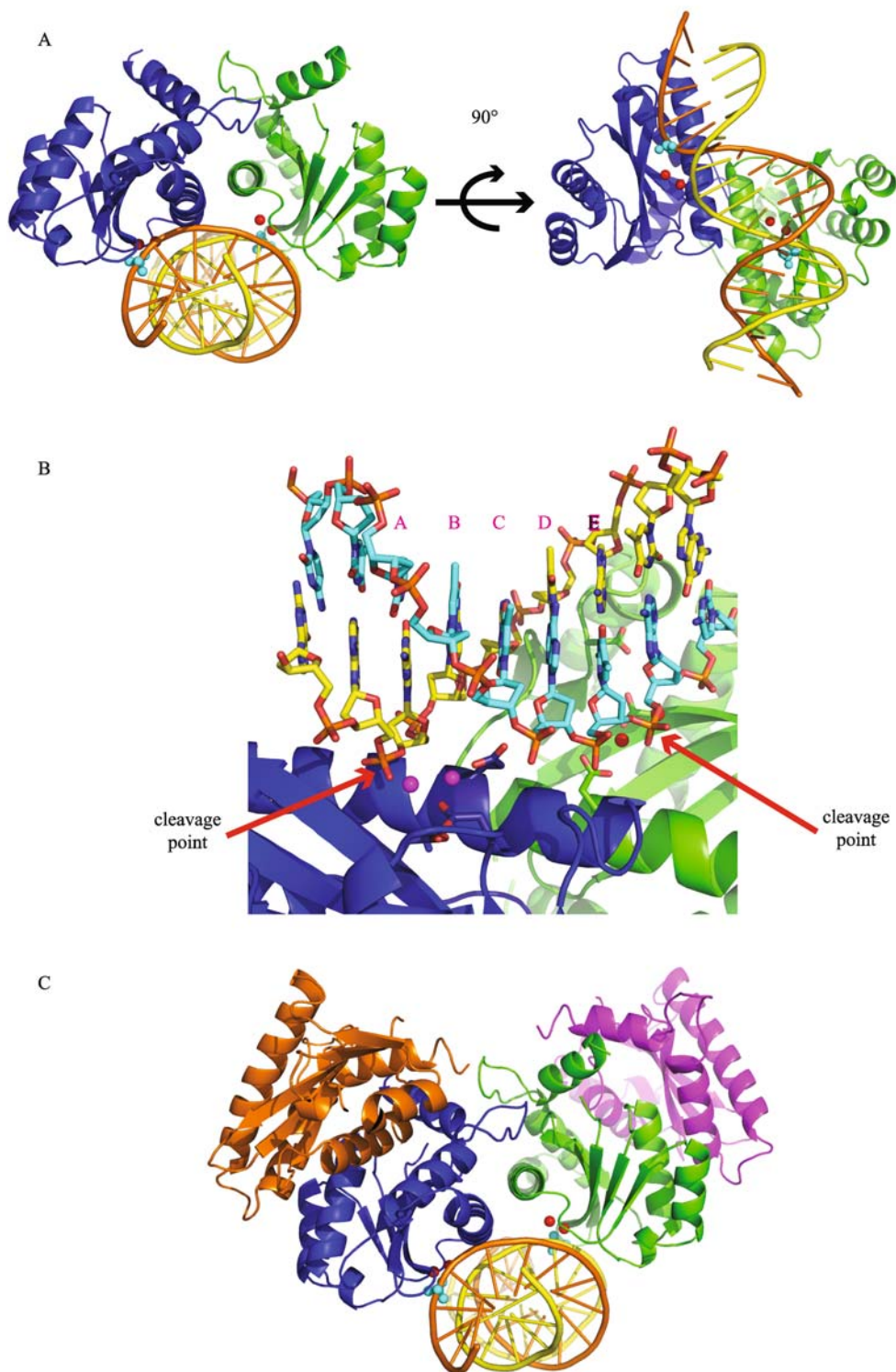
Figure 3. Our proposed model of the interaction of integrase with target DNA. (A) Cartoon representation of the face-to-face dimer binding with target DNA. The two monomers are colored blue and green. Two magnesium ions in each monomer are shown as red spheres. Each phosphate molecule is shown as cyan sphere. The double helices of the DNA template are colored orange and yellow, respectively. The base pairs are represented by sticks. (B) Details of the binding interactions of the target DNA in the active sites of the dimer. The DNA template is represented using sticks. The carbon atoms are colored cyan and yellow in the different chains. The oxygen, nitrogen and phosphorus atoms are colored red, blue and orange, respectively. Magnesium ions are shown as red and magenta spheres. (C) Cartoon representation of BIV integrase CCD tetramer binding with target DNA. Four CCDs are colored as orange, blue, green and magenta, respectively.
