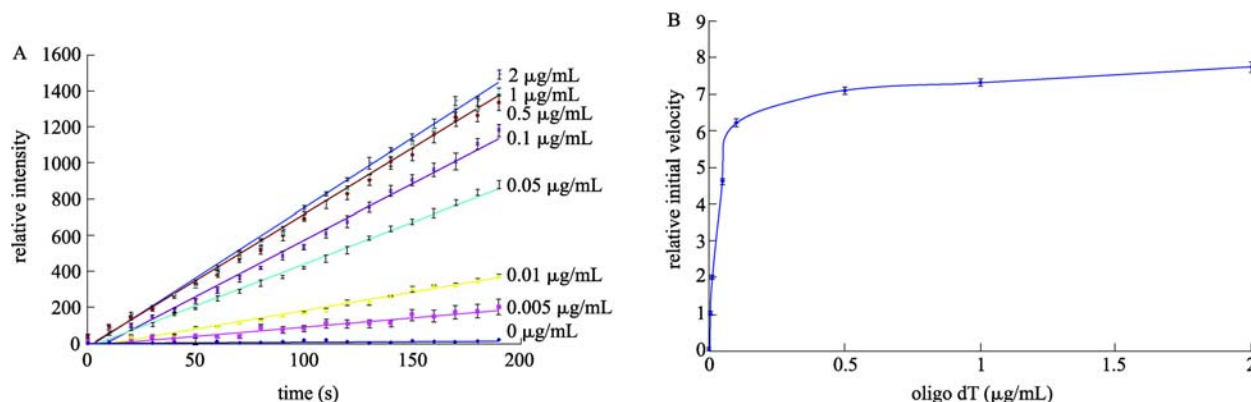
Figure 3. Effects of oligo (dT) 18 concentration on activity. (A) Various concentrations of oligo (dT) 18 were added; the HIV-RT concentration is 1.25 \mu\text{g}/\text{mL} , other conditions and parameters are as described for Fig. 1A. Results shown are the average of 5 independent experiments ( n = 5 ). (B) Polymerase activity increased with primer concentration, with indications of saturation at the maximum tested (2 \mu\text{g}/\text{mL} ).
