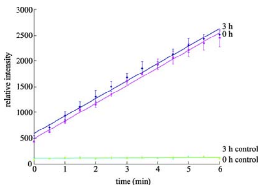
Figure 4. Pre-incubation of HIV-RT. HIV-RT was pre-incubated with polyA and oligo (dT) 18; the HIV-RT concentration is 1.25 mg/mL, other conditions and parameters are as described for Fig. 1A. No obvious increase in signal was observed within 3 h of pre-incubation. Data were collected from three independent reactions ( n = 3 ) for 0.1 s every 30 s during a 6-min reaction.
