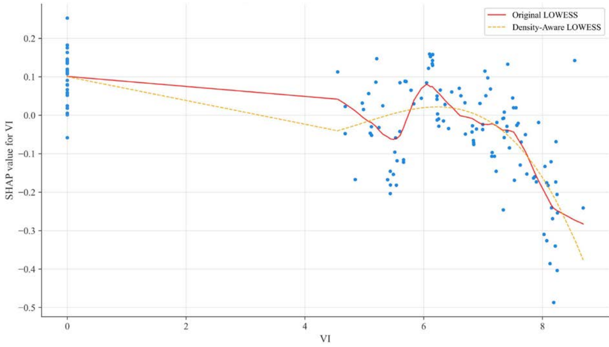
Supplementary Fig. 14 SHAP dependence plot of VI (density-aware fitting). © Xiaoju Li
