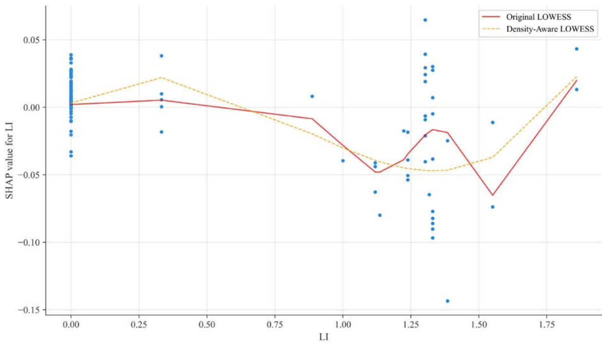
Supplementary Fig. 11 SHAP dependence plot of LI (density-aware fitting). © Xiaoju Li
