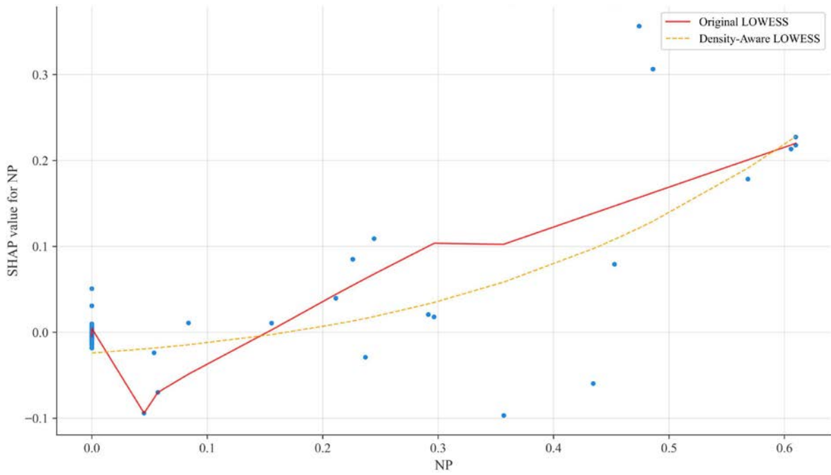
Supplementary Fig. 15 SHAP dependence plot of NP (density-aware fitting). © Xiaoju Li
