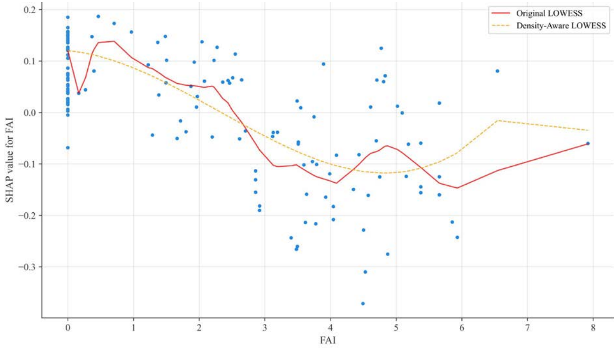
Supplementary Fig. 4 SHAP dependence plot of FAI (density-aware fitting). © Xiaoju Li
