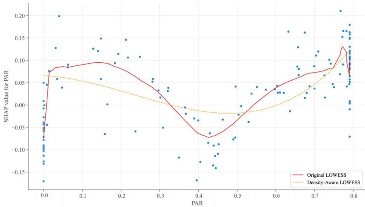
Supplementary Fig. 19 SHAP dependence plot of PAR (density-aware fitting). © Xiaoju Li
