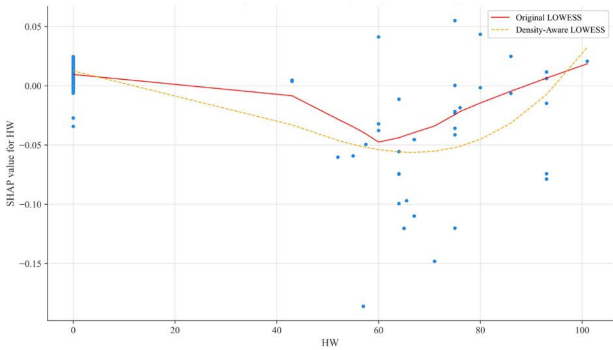
Supplementary Fig. 2 SHAP dependence plot of HW (density-aware fitting). © Xiaoju Li
