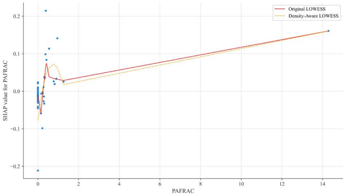
Supplementary Fig. 17 SHAP dependence plot of PAFRAC (density-aware fitting). © Xiaoju Li
