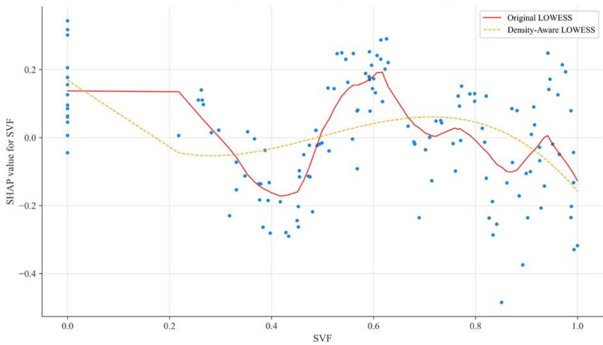
Supplementary Fig. 3 SHAP dependence plot of SVF (density-aware fitting). © Xiaoju Li
