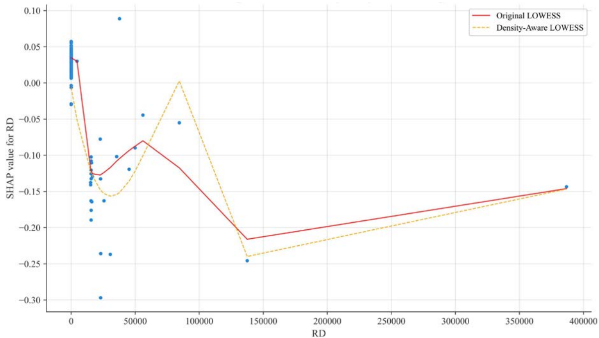
Supplementary Fig. 6 SHAP dependence plot of RD (density-aware fitting). © Xiaoju Li
