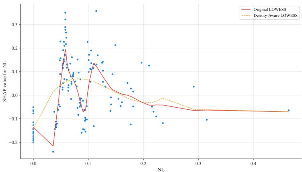
Supplementary Fig. 7 SHAP dependence plot of NL (density-aware fitting). © Xiaoju Li
