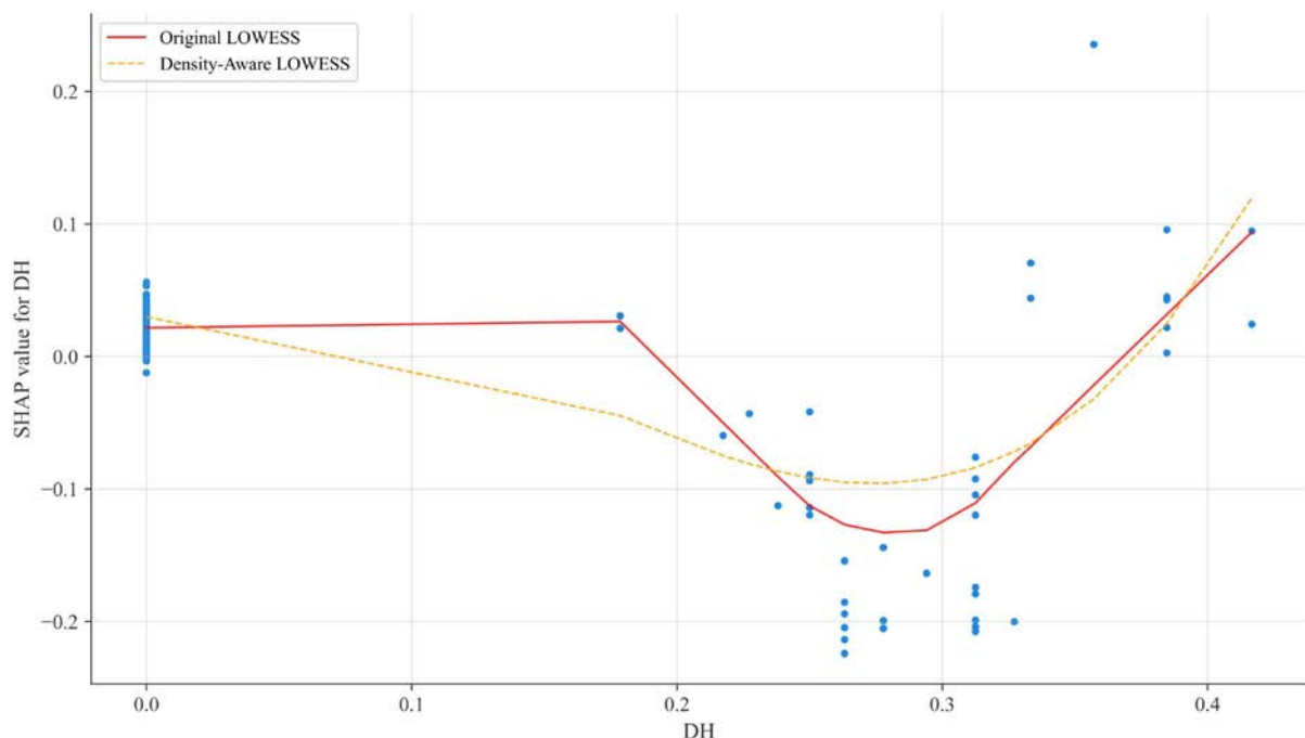
Supplementary Fig. 1 SHAP dependence plot of DH (density-aware fitting). © Xiaoju Li
