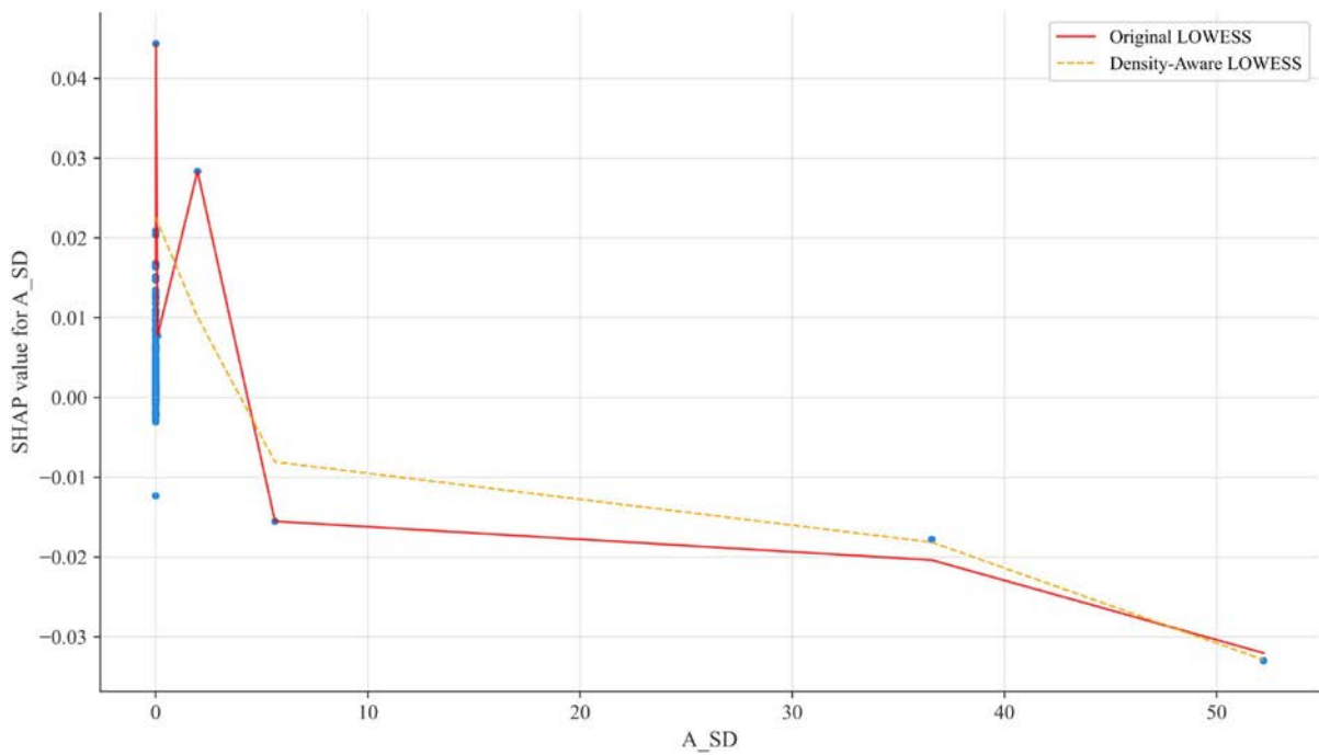
Supplementary Fig. 5 SHAP dependence plot of A_SD (density-aware fitting). © Xiaoju Li
