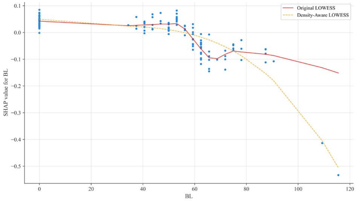
Supplementary Fig. 8 SHAP dependence plot of BL (density-aware fitting). © Xiaoju Li
