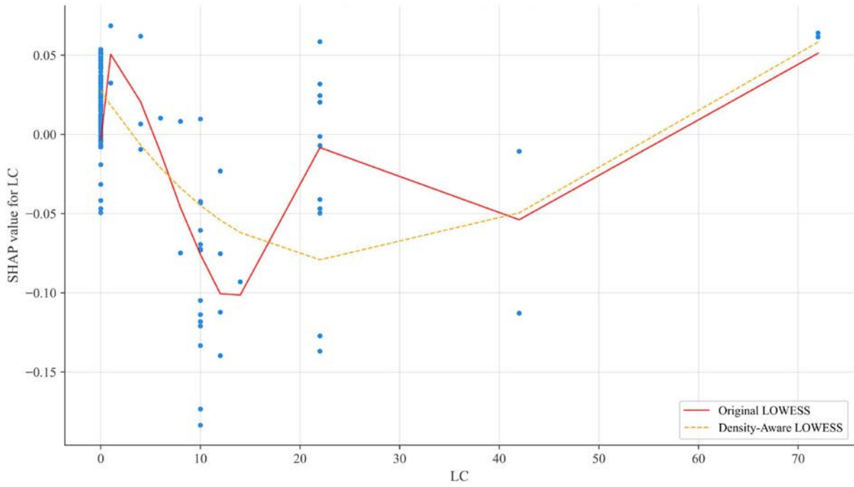
Supplementary Fig. 10 SHAP dependence plot of LC (density-aware fitting). © Xiaoju Li
