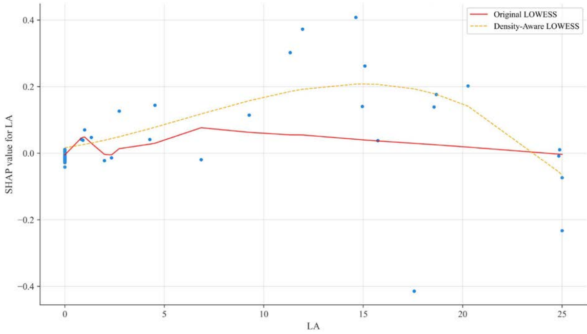
Supplementary Fig. 16 SHAP dependence plot of LA (density-aware fitting). © Xiaoju Li
