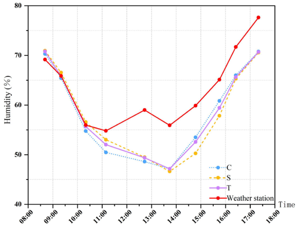
Supplementary Fig. 20 Comparison of average humidity in three types of spaces across different time periods with that at meteorological stations. © Xiaoju Li
