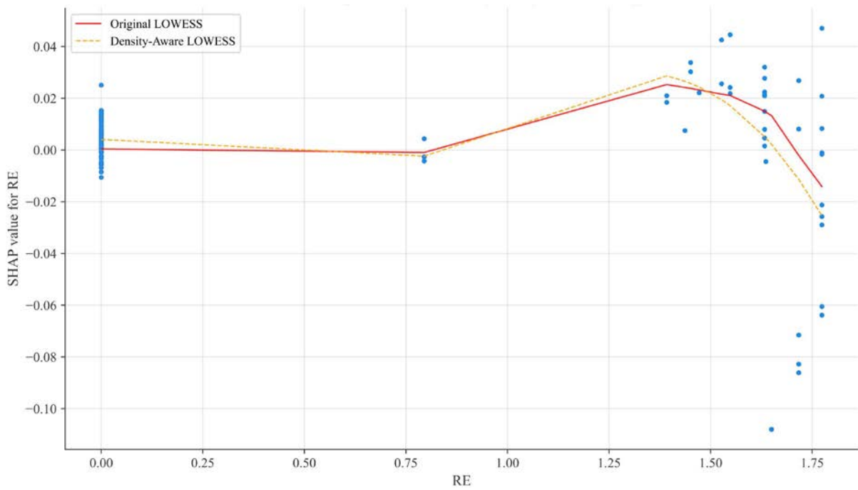
Supplementary Fig. 13 SHAP dependence plot of RE (density-aware fitting). © Xiaoju Li
