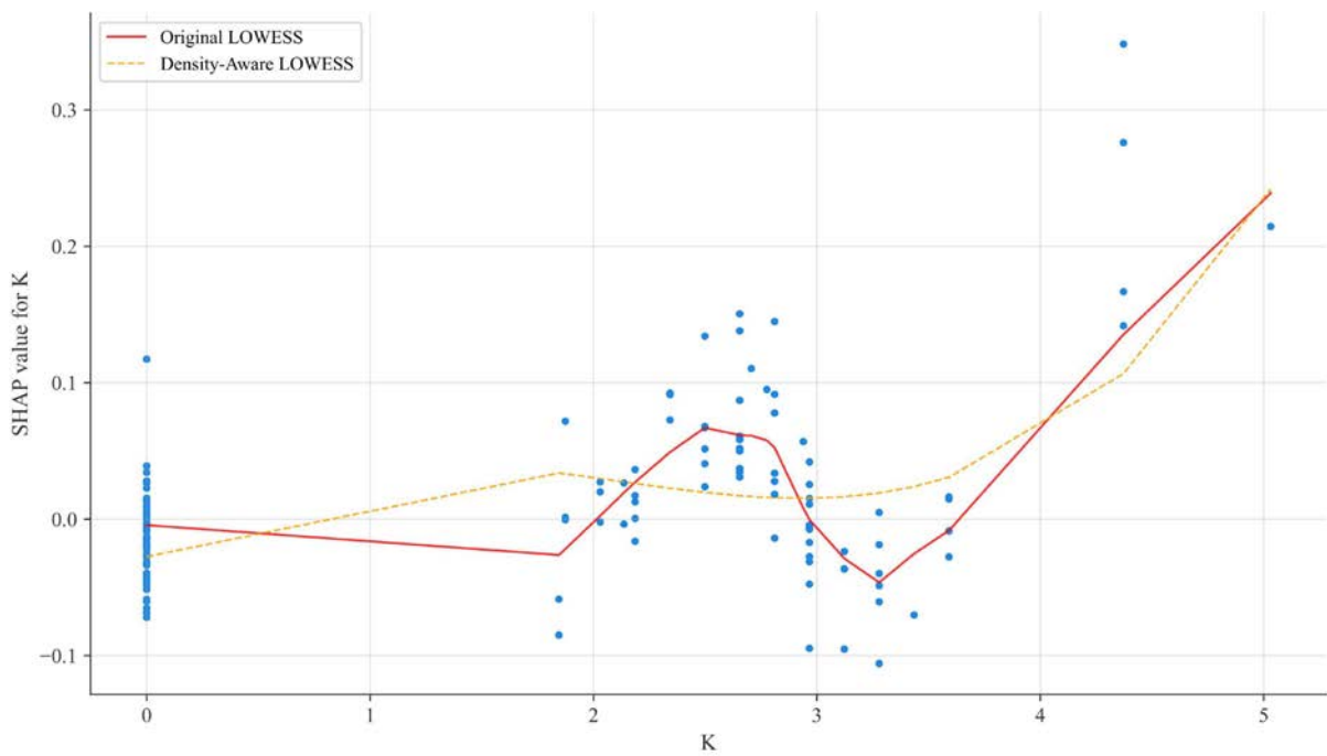
Supplementary Fig. 9 SHAP dependence plot of K (density-aware fitting). © Xiaoju Li
