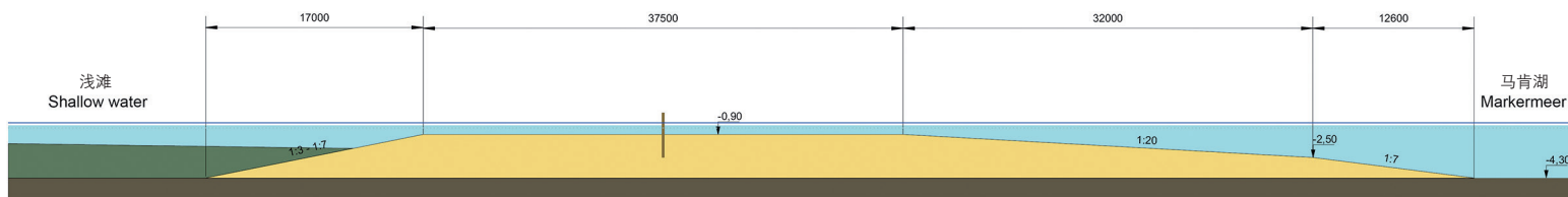
Compartment dam opening up section 间隔式水坝展开剖面图
