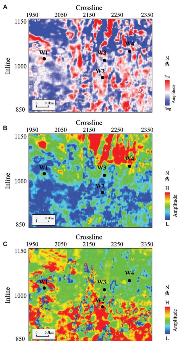
Figure 7. Seismic attribute slices extracted along H1 based on the post-stacked field data. (A) Seismic amplitude attribute. (B) Root mean square attribute. (C) Instantaneous frequency attribute.
