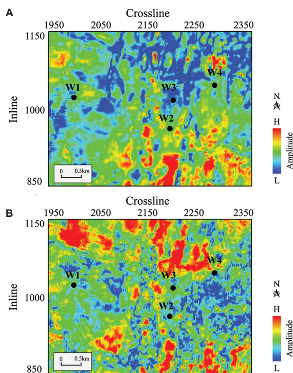
Figure 8. Constant frequency components extracted along H1 by using the S-transform; (A) low-frequency component and (B) high-frequency component.
