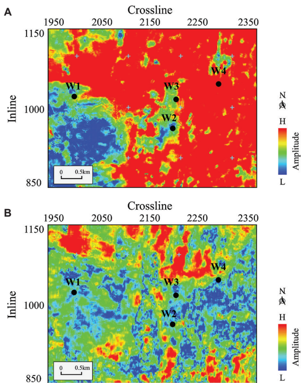
Figure 9. Constant frequency components extracted along H1 by using the unscaled S-transform; (A) low-frequency component and (B) high-frequency component
