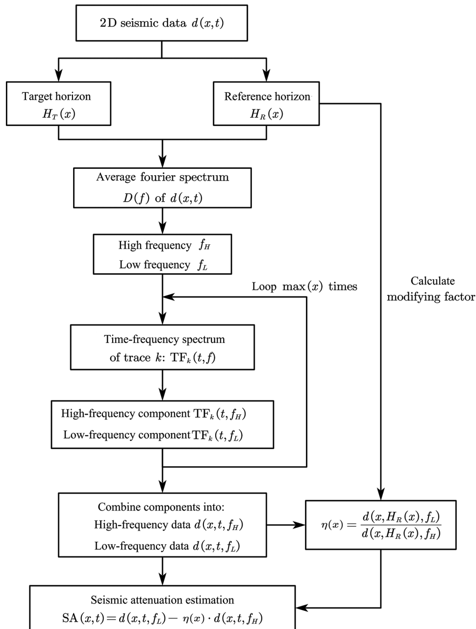
Figure 1. The proposed workflow of seismic attenuation characterization based on the proposed unscaled generalized S-transform. Abbreviations: 2D: Two-dimensional; SA: Seismic attenuation.
