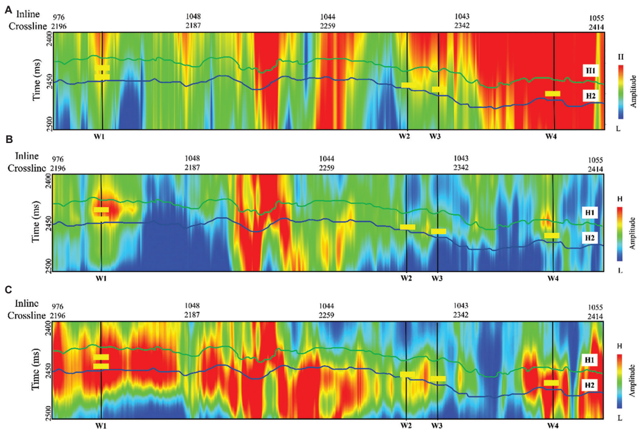
Figure 6. Seismic attenuation estimation for two-dimensional post-stacked field data in Figure 4, calculated by using (A) S-transform, (B) Unscaled S-transform, and (C) Unscaled generalized S-transform
