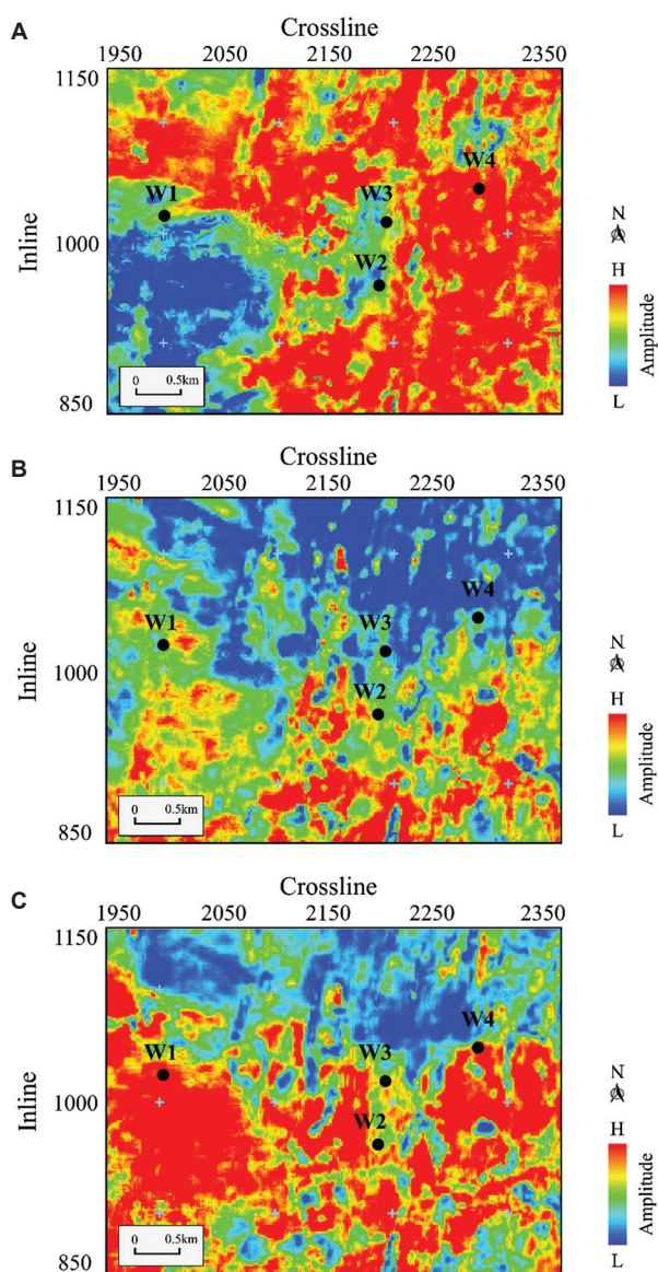
Figure 11. Seismic attenuation slices of H1 in 3D field data calculated by using (A) S-transform, (B) unscaled S-transform, and (C) unscaled generalized S-transform, respectively
