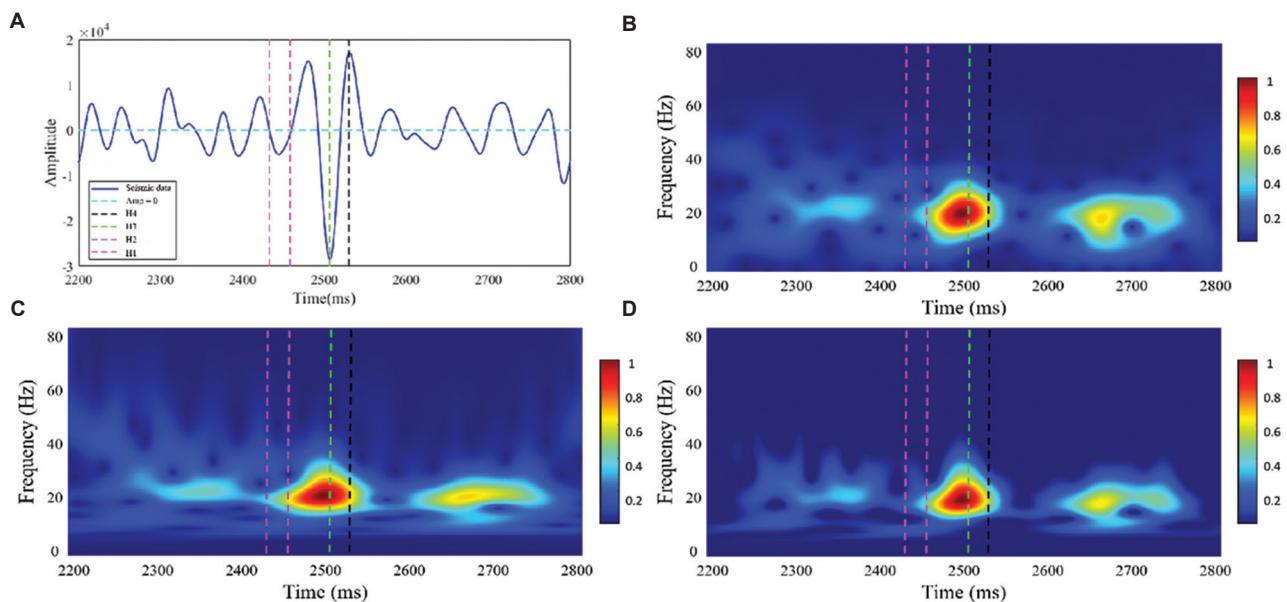
Figure 4. A representative seismic trace and its time-frequency spectra. (A) A representative seismic trace located near Well A and its time–frequency transform results calculated using (B) S-transform, (C) Unscaled S-transform, and (D) Unscaled generalized S-transform. The black, green, and two pink dashed lines indicate horizon H4, H3, H2, and H1, where the interpreted reservoir is located between H1 and H2.
