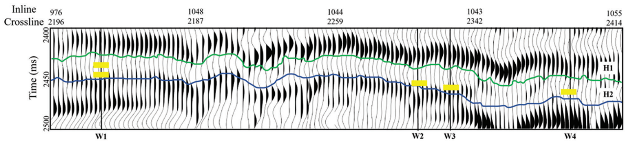
Figure 5. Two-dimensional post-stacked field data with four borehole locations. The green and dark blue solid curves present two interpreted horizons: H1 and H2. The yellow blocks indicate the location of the interested reservoirs.
