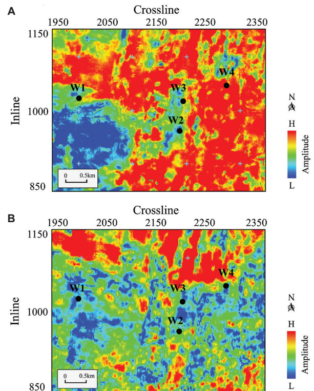
Figure 10. Constant frequency components extracted along H1 by using the unscaled generalized S-transform; (A) low-frequency component and (B) high-frequency component
