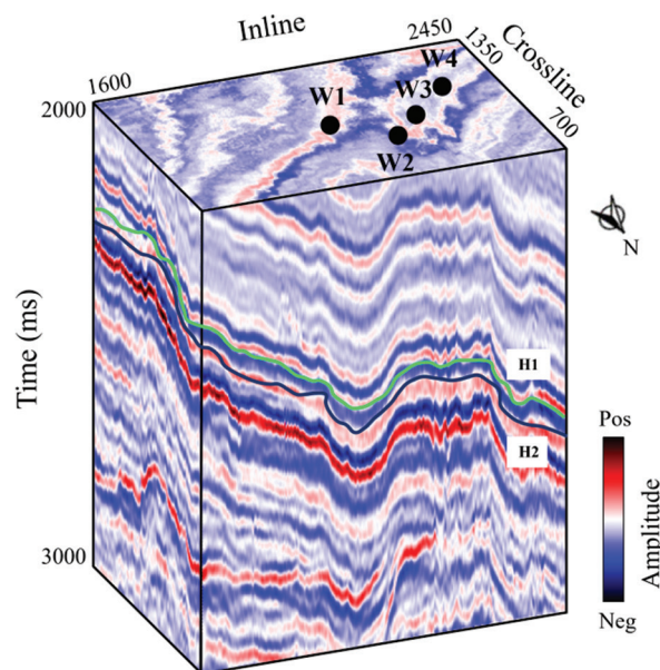
Figure 2. The three-dimensional post-stacked seismic data, located at the Ordos Basin, Northwest China, where W1, W2, W3, and W4 indicate four productive wells. The green and dark blue solid curves present two interpreted horizons: H1 and H2.
