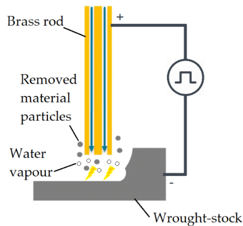
Figure 1. Schematic of the EDM discharge process and material removal [10].
