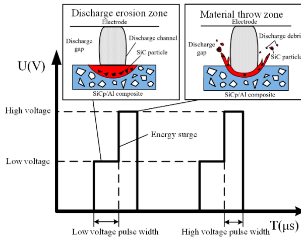
Figure 4. High- and low-voltage composite waveform [76].
