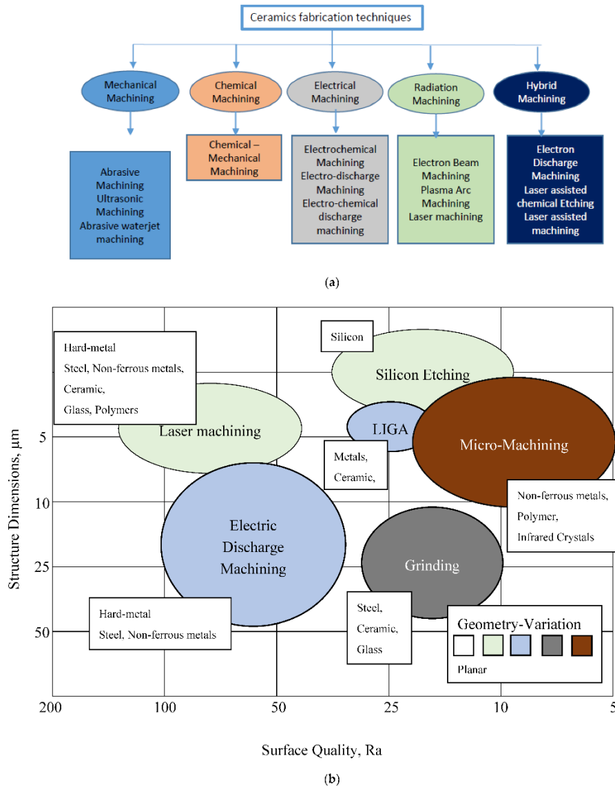
Figure 5. (a) Ceramic fabrication techniques, (b) EDM and micro-EDM relative to other manufacturing processes on CMC [77].
