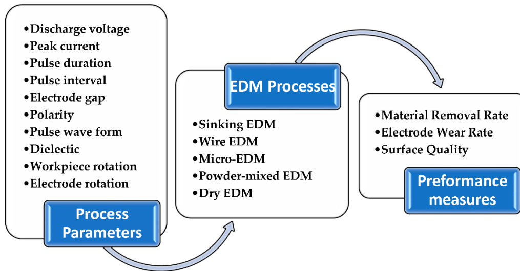
Figure 2. The processes of EDM and their process parameters and performance measures [22].
