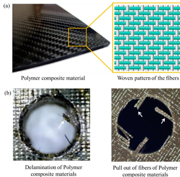
Figure 3. (a) Polymer composite materials and woven patterns of fibres of the reinforcement phase; and (b) delamination and pull out of fibres during the drilling of polymer composite materials [64].
