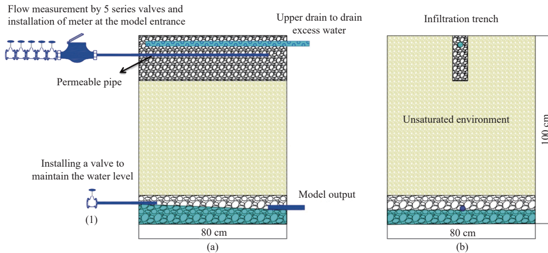
Fig. 1 A simple schematic of the laboratory model
