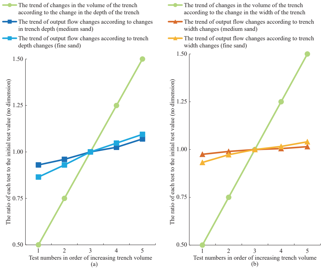
Fig. 5 Examining the changes in the volume of the trench and the changes in the output flow in medium sand and fine sand
