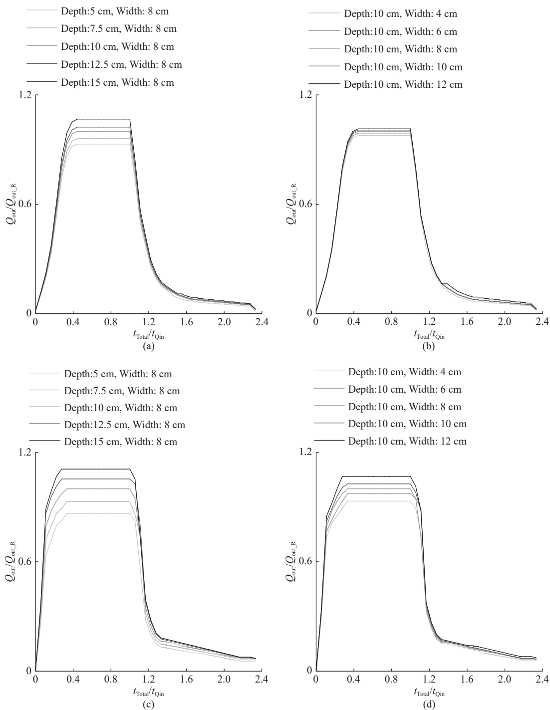
Fig. 4 The effect of changes in channel dimensions on flow output in the physical model
