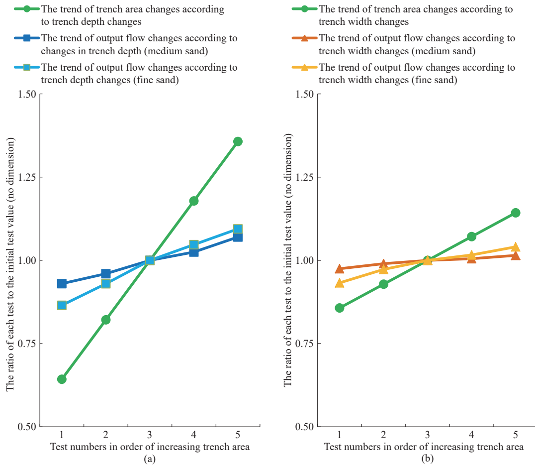
Fig. 6 Examining the changes in the wetted surface of the trench and the changes in the output flow in medium sand and fine sand
