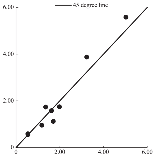
Fig. 8 Comparison of the observed values of leakage from the channel with its calculated values from the equation against the 45-degree line
