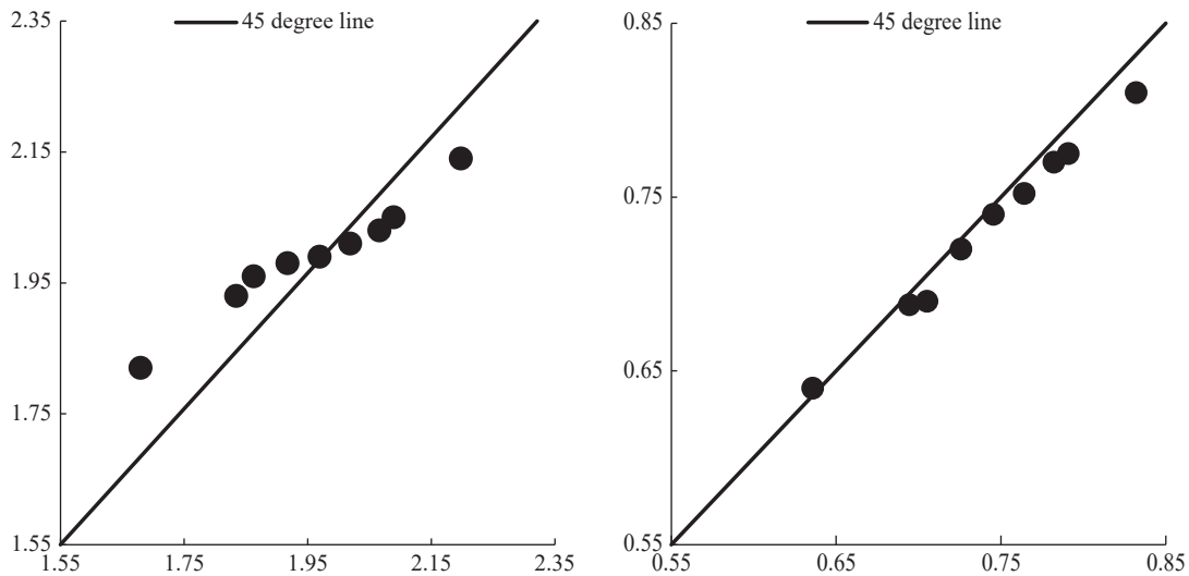
Fig. 7 Comparison of observed values of Q_{out} and calculated values of Q_{out} from the provided equation (a) for medium sand materials against the 45-degree line; (b) for fine sand materials against the 45-degree line.
