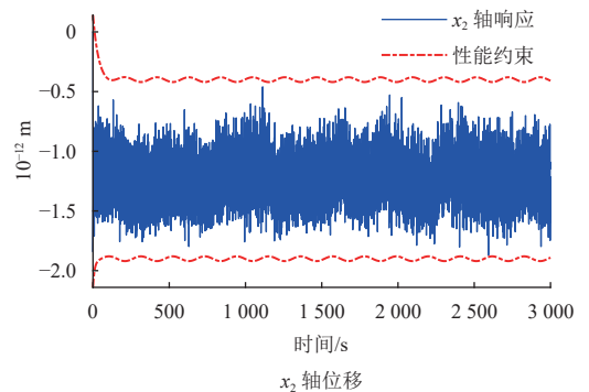
Fig. 4 Displacement response compared with QFT-based scheme
