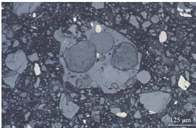
图2 Apollo 17月壤的颗粒形态 [11] Fig. 2 Granular morphology of Apollo 17 lunar soil [11]
