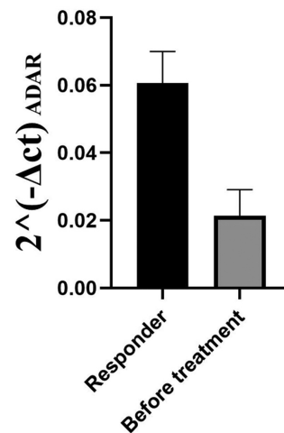
Fig. 3 Comparison of ADAR expression in responders after 1 year follow-up with before starting drug therapy. Assessment of 2^{-\Delta CT} in responders comparing expression levels before beginning treatment and after a year follow-up showed elevated rates in ADAR expression in response to drug therapy. ADAR, Adenosine deaminase, RNA-specific.
