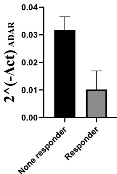
Fig. 2 Relative ADAR expression rates between two groups of drug response. Quantitative real-time PCR was performed to measure expression rates and 2^{-\Delta CT} was used to show fold change analysis on the mean values. Responders and nonresponders were compared and 2^{-\Delta CT} was higher in nonresponders. Hence, ADAR had more expression in nonresponder group compared with responders. ADAR, Adenosine deaminase, RNA-specific; PCR, polymerase chain reaction.
