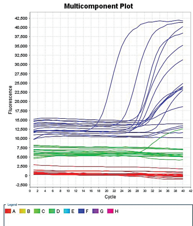
Fig. 2 Real-time polymerase chain reaction (PCR) multicomponent graph showing HPV 16 (blue line), HPV 18 (green line), and internal control (red line) expression in cases and control.
