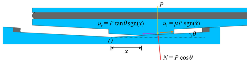
Fig. 3 Theoretical analysis model for MPCFS.
