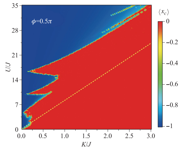
Fig. 8 Phase diagram of transition to self-trapping with rescaled tunneling amplitude K/J and rescaled interaction strength U/J at \phi = 0.5\pi . The dashed line indicates the simple analytical results from Eq. (10) with considering a double-well potential approximation.
