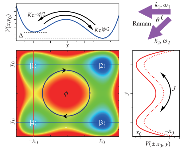
Fig. 1 Schematic diagram showing the system under consideration. The quadruple-well potential can be equivalently with a four-site plaquette in an optical lattice, which was achieved by applying superlattice potentials along both the x - and y -directions, so that all dynamics is restricted to four sites without any coupling between plaquettes. The potential along the y -direction is symmetric, and the bare tunneling occurs along the y -direction with amplitude J . The potential along the x -direction generates a tilted potential with amplitude \Delta , which inhibits the bare tunneling along the x -direction. Then, an additional pair of lasers with wave vectors \mathbf{k}_{1,2} and frequency difference \omega_1 - \omega_2 = \Delta/\hbar induced resonant tunneling along the x -direction with complex amplitude K(\mathbf{R}) whose phase depends on position.
