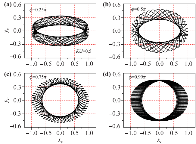
Fig. 5 Various quasi-periodic cyclotron orbits induced by synthetic gauge fields \phi . The surrounding properties of quasi-periodic cyclotron orbits cannot be changed by synthetic gauge fields. The volume of the phase space is affected by the synthetic gauge fields \phi .
