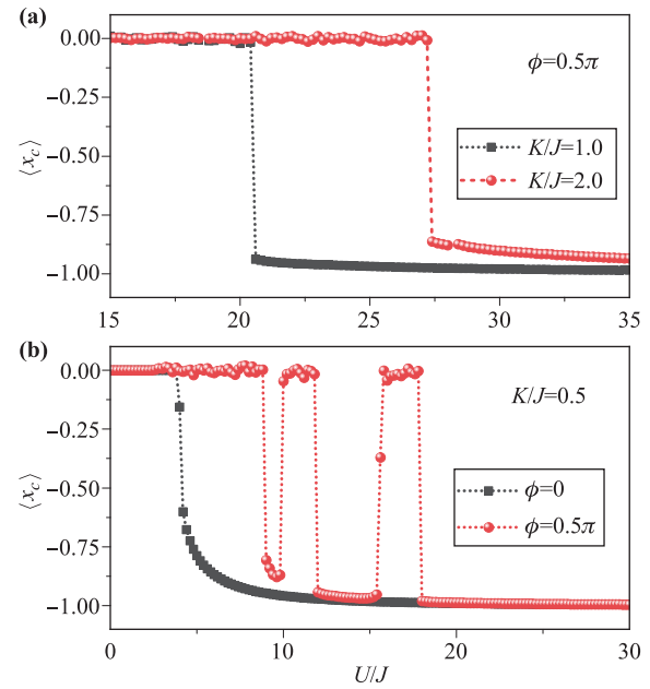
Fig. 7 The average of x_c versus the rescaled interaction strength U/J : (a) for different K/J at \phi = 0.5\pi , (b) for different \phi at K/J = 0.5 .
