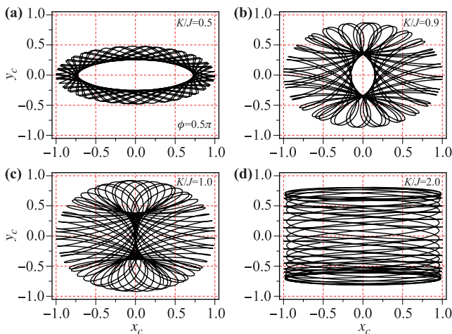
Fig. 4 Various quasi-periodic cyclotron orbits induced by rescaled tunneling amplitude K/J . The surrounding properties of quasi-periodic cyclotron orbits are significantly affected by tunneling amplitude.
