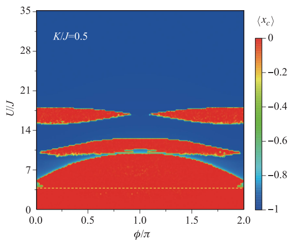
Fig. 9 Phase diagram of transition to self-trapping with synthetic gauge fields \phi and rescaled atomic interaction strength U/J at K/J = 0.5 . The dashed line indicates the simple analytical results from Eq. (10) with considering a double-well potential approximation.
