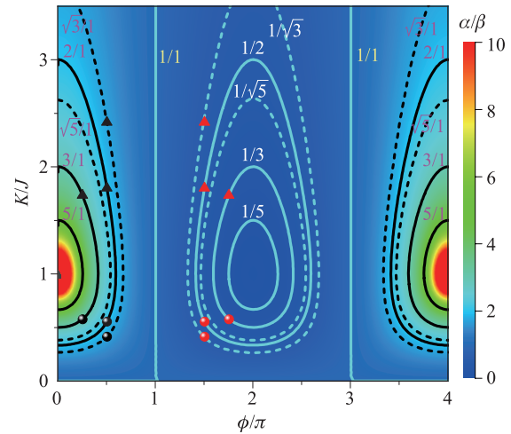
Fig. 2 Contour plot of the rate \alpha/\beta as a function of synthetic gauge fields \phi/\pi and rescaled tunneling amplitude K/J . Periodic and quasi-periodic dynamic cyclotron orbits can be analyzed by the principle of commensurability between \alpha and \beta . When these two frequencies \alpha and \beta are commensurable, the dynamics of the system presents periodic cyclotron orbits. However, when the two frequencies are incommensurable, the dynamics of the system presents quasi-periodic cyclotron orbits. Typical frequency ratios are shown in the figure.
