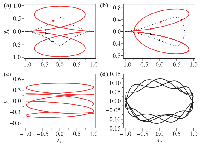
Fig. 3 The typical periodic and quasi-periodic orbits, the direction of the arrow represents the evolution direction of the orbit. (a) Periodic orbits for \alpha/\beta = 1/2 and \alpha/\beta = 2/1 . (b) Periodic orbits for \alpha/\beta = 1/3 and \alpha/\beta = 3/1 . In (a), the red solid line with the black arrow corresponds to the black triangle on the \alpha/\beta = 2/1 line in Fig. 2; the black dashed line with the black arrow corresponds to the black point on the \alpha/\beta = 2/1 line in Fig. 2; the red solid line with the red arrow corresponds to the red triangle on the \alpha/\beta = 1/2 line in Fig. 2; the black dashed line with the red arrow corresponds to the red point on the \alpha/\beta = 1/2 line in Fig. 2. (b) has an analogous correspondence for \alpha/\beta = 3/1, 1/3 . (c, d) Quasi-periodic orbits for \alpha/\beta = \sqrt{3}/1 at \phi = 0.5\pi . (c) for the quasi-periodic cyclotron orbit corresponds to the black triangle on the \alpha/\beta = \sqrt{3}/1 line in Fig. 2. (d) for the quasi-periodic cyclotron orbit corresponds to the black point on the \alpha/\beta = \sqrt{3}/1 line in Fig. 2.
