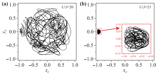
Fig. 6 Complex dynamic cyclotron orbit with atomic interaction. (a) U/J = 20 , (b) U/J = 21 . The other parameters are \phi = 0.5\pi and K/J = 1 . The inset in (b) is enlarged for more clear display.
