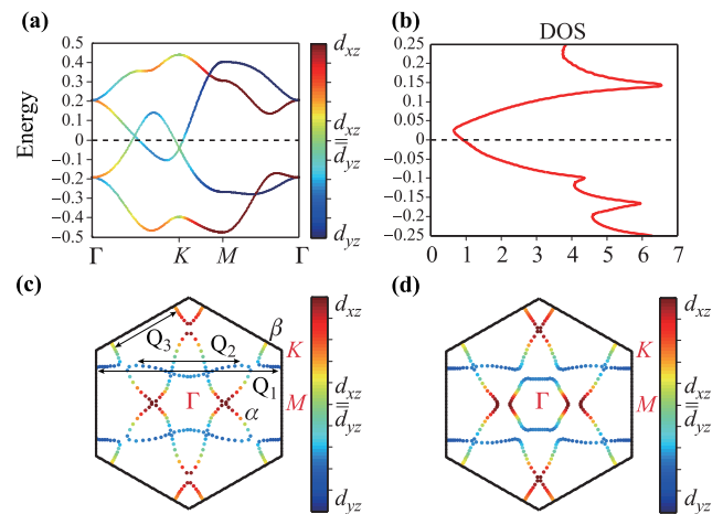
Fig. 1 The orbital characters of bands are represented by different colors. (a) Band dispersion of tight-binding model based on d_{xz} and d_{yz} orbitals of Ni atoms. (b) The corresponding density of states (DOS) for NiPS 3 . The van Hove singularities (vHs) are above the Fermi level near 0.14 eV. Orbital resolved Fermi surface with two different electron fillings, \delta = 0.3 (c) and \delta = 0.35 (d) per Ni atom with respect to the half-filling. The type-II vHs appear along \Gamma - M line or \Gamma - K line which are not at TRIM points.
