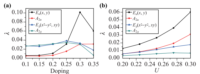
Fig. 3 Leading pairing strengths in spin singlet [ E_g ( d -wave), A_{2g} ( I -wave)] and triplet [ E_u ( p -wave), A_{2u} ( f -wave)] channels for superconducting states with different electron dopings \delta at U = 0.3 and J/U = 0.2 in (a). The pairing strengths with \delta = 0.35 per Ni atom at J/U = 0.2 are plotted in (b).
