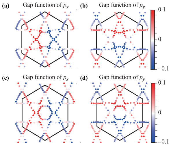
Fig. 4 The gap functions p_x and p_y of leading triplet pairings with U = 0.3 and J/U = 0.2 at \delta = 0.3 (a, b) and \delta = 0.35 per Ni atom (c, d).
