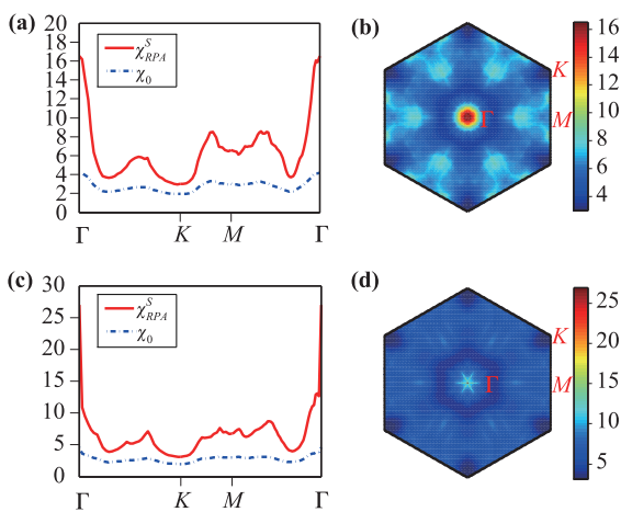
Fig. 2 Susceptibilities for different electron doping. The bare susceptibilities \chi_0 and RPA spin susceptibilities \chi_{RPA}^s along high-symmetry lines for \delta = 0.3 (a) and \delta = 0.35 (c) per Ni atom (near type-II vHs). The corresponding RPA spin susceptibilities in 2D Brillouin zone are shown in (b) and (d) with U = 0.3 and J/U = 0.2 .
