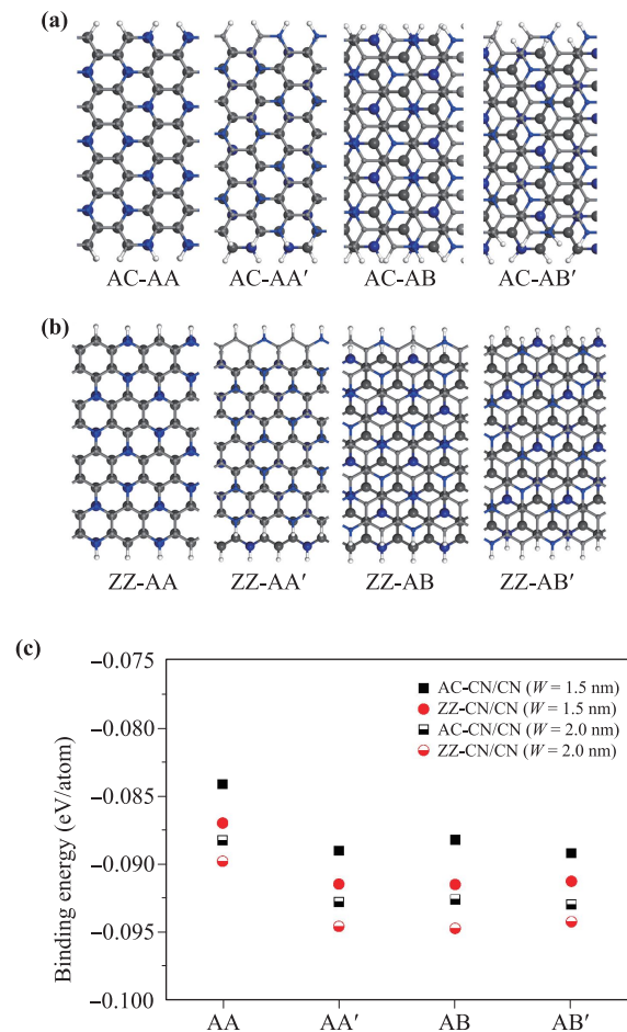
Fig. 2 (a, b) Structure illustration of (a) bilayer AC-CN/CN and (b) bilayer ZZ-CN/CN with AA-, AA'-, AB-, or AB'-stacking. The grey, blue and white balls represent C, N, and H atoms, respectively. Besides, the lower atoms have deeper color and larger size than upper atoms. (c) Binding energies of four stacking orders with different edge configurations and widths. The black solid square and black hollow square stand for AC-CN/CN with the width of 1.5 nm and 2.0 nm, respectively. And the red solid circle and red hollow circle represent ZZ-CN/CN with the width of 1.5 nm and 2.0 nm, respectively.
