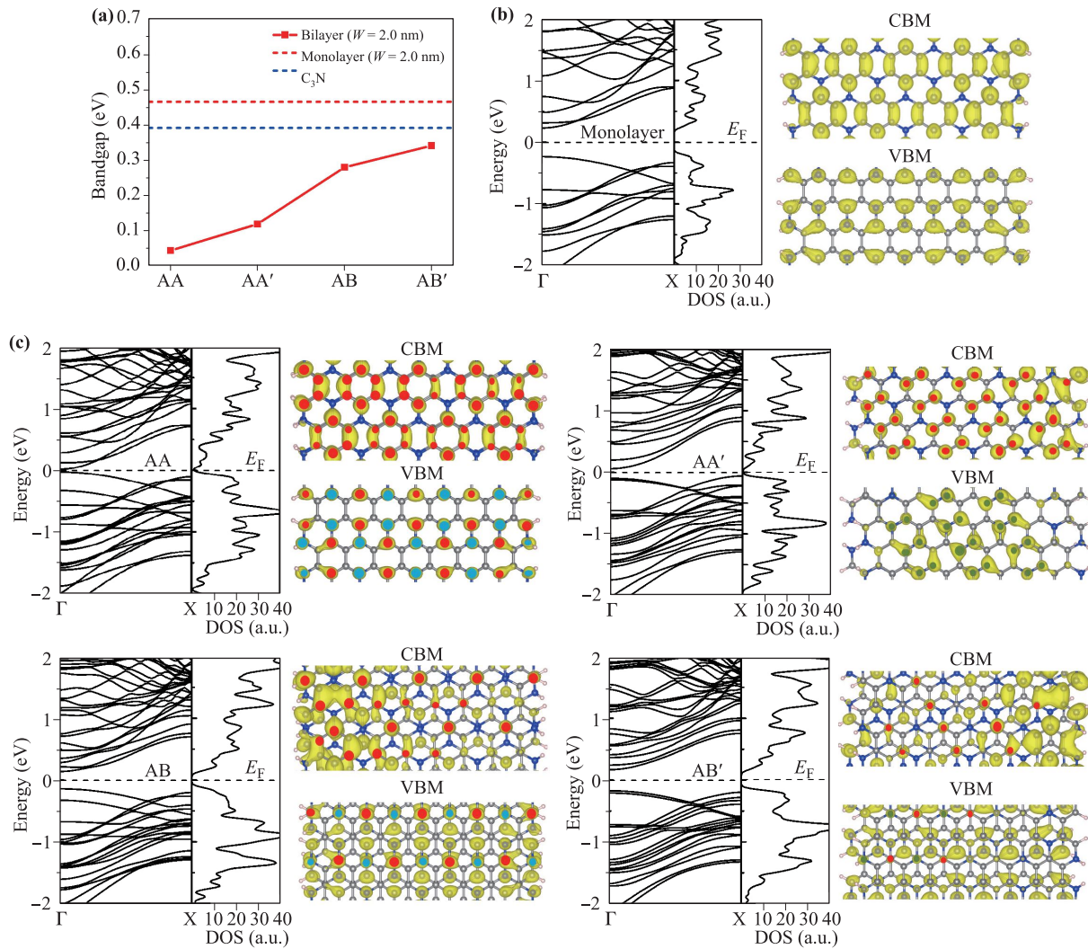
Fig. 3 (a) The bandgaps of bilayer AC-CN/CN with AA-, AA'-, AB-, and AB'-stacking, which is shown by red solid line. The red and blue dashed lines exhibit the bandgaps of monolayer AC-CN/CN and C_3N sheet, respectively. (b) The band structure, density of states (DOS) and partial charge (CBM and VBM) of monolayer AC-CN/CN. (c) The band structure, DOS and partial charge (CBM and VBM) of bilayer AC-CN/CN with AA-, AA'-, AB-, and AB'-stacking. The red, blue and green circles stand for p_z orbital overlap contributed by C/C, N/N, and C/N atoms.
