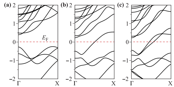
Fig. S7 The band structure of monolayer (a) ZZ-CN/CN with the width of 1.3 nm, (b) ZZ-CC/CN with the width of 1.5 nm and (c) ZZ-CC/CC with the width of 1.5 nm. The red dashed lines display the position of the Fermi level.
