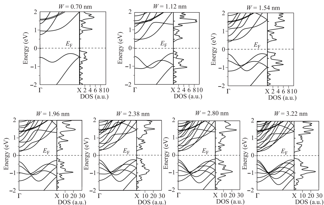
Fig. S6 The band structure and DOS of monolayer ZZ-CN/CN nanoribbons with different widths.
