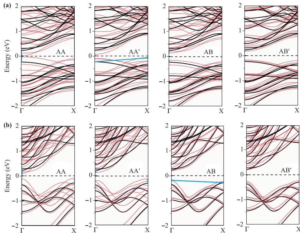
Fig. S8 (a) The difference of band structure between bilayer and monolayer AC-CN/CN with the width of 2 nm. (b) The difference of band structure between bilayer and monolayer ZZ-CN/CN with the width of 2 nm. The band structure of the monolayer is shown by black lines, and the bilayer is shown by red lines. The blue arrow represents the energy shift.
