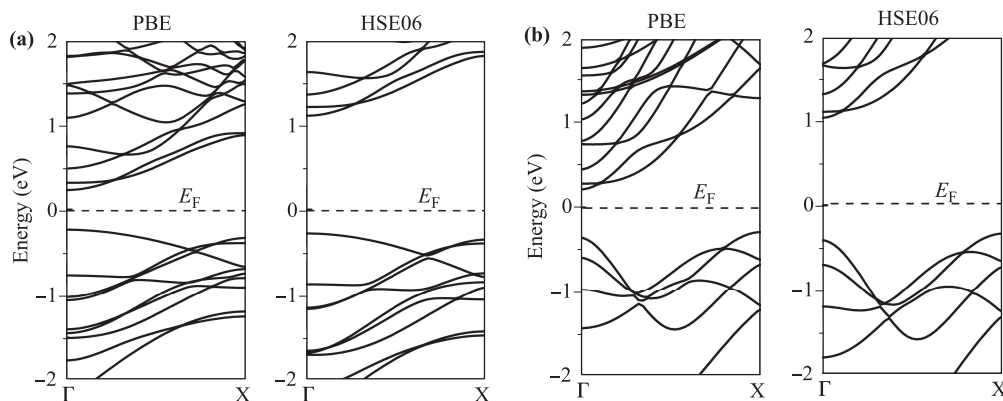
Fig. S9 The band structure of (a) AC-CN/CN and (b) ZZ-CN/CN monolayer with the width of 2 nm calculated by PBE and HSE06 functionals.
