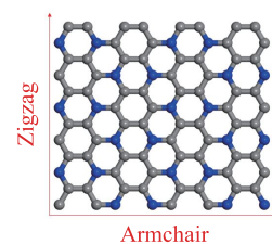
Fig. S1 The top view of C 3 N sheet. The grey and blue balls represent C and N, respectively.
