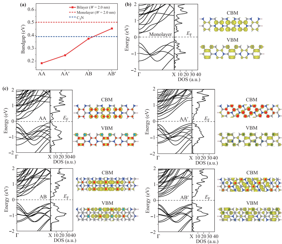
Fig. 4 (a) The bandgaps of bilayer ZZ-CN/CN with four stacking orders, which is shown by red solid line. The red and blue dashed line show the bandgaps of monolayer ZZ-CN/CN and C_3N sheet. (b, c) The band structure, DOS and partial charge (CBM and VBM) of (b) monolayer ZZ-CN/CN and (c) bilayer ZZ-CN/CN heterostructure with different stacking orders. The red, blue and green circles represent p_z orbital overlap of CC, NN, and CN atoms, respectively.
