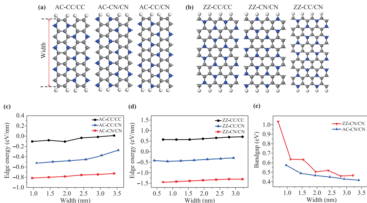
Fig. 1 (a, b) The atomistic configurations of (a) AC- C_3N NNRs and (b) ZZ- C_3N NNRs with three types of edge configurations. The grey, blue and white balls represent C, N and H atoms, respectively. (c, d) The edge energies of (c) AC- C_3N NNRs and (d) ZZ- C_3N NNRs as a function of the ribbon width. (e) The bandgaps of ZZ-CN/CN (red line) and AC-CN/CN (blue line) as a function of the ribbon width.
