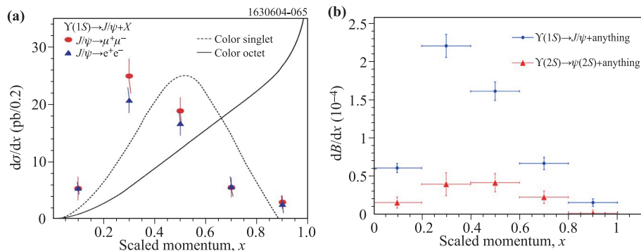
Fig. 5 (a) The differential cross sections in x for \Upsilon(1S) \rightarrow J/\psi + \text{anything} from CLEO [56]. (b) The differential branching fractions of \Upsilon(1S) inclusive decays into the J/\psi and \psi(2S) from Belle [57].
