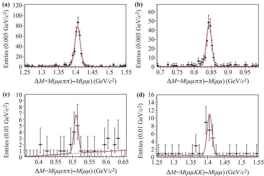
Fig. 21 The \Delta M distributions for (a) \Upsilon(5S) \rightarrow \Upsilon(1S)\pi^+\pi^- , (b) \Upsilon(5S) \rightarrow \Upsilon(2S)\pi^+\pi^- , (c) \Upsilon(5S) \rightarrow \Upsilon(3S)\pi^+\pi^- , and (d) \Upsilon(5S) \rightarrow \Upsilon(1S)K^+K^- from Belle [171]. The solid red lines show the best fits to the data, while the dashed red lines show the backgrounds.
