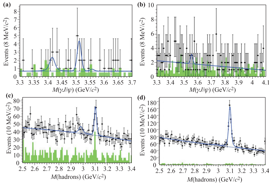
Fig. 7 The \gamma J/\psi invariant mass distributions in the (a) \Upsilon(1S) and (b) \Upsilon(2S) decays, and invariant mass spectra for \eta_c candidates in the (c) \Upsilon(1S) and (d) \Upsilon(2S) decays from Belle [73, 74]. The shaded histograms in (a) and (b) are from the normalized J/\psi sidebands, and the shaded histograms (not normalized) in (c) and (d) are from the continuum contributions.
