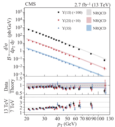
Fig. 27 The differential \Upsilon(1S, 2S, 3S) cross sections times dimuon branching fractions as a function of p_T at \sqrt{s} = 13 \text{ TeV} in the rapidity range of |y| < 1.2 from CMS [203]. The bands show the predictions by NLO NRQCD [204, 205]. The middle panel shows the ratios of measurements to the theory, and the lower panel shows the ratios of cross sections measured at \sqrt{s} = 13 \text{ TeV} to those measured at 7 \text{ TeV} [201].
