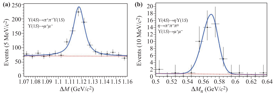
Fig. 19 The \Delta M (a) and \Delta M_\eta (b) distributions for \Upsilon(4S) \rightarrow \pi^+\pi^-\Upsilon(1S) and \Upsilon(4S) \rightarrow \eta\Upsilon(1S) from Belle [168]. The data, best fits to them, and background contributions are shown by the dots with error bars, solid blue lines, and dashed red lines, respectively.
