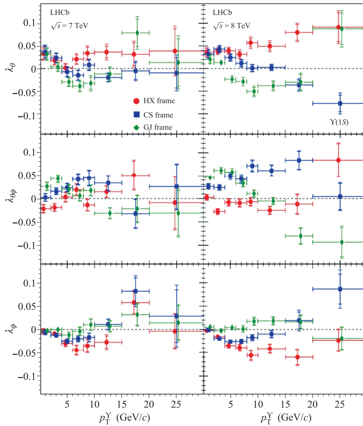
Fig. 29 The polarization parameters \lambda_\theta (top), \lambda_{\theta\phi} (middle), and \lambda_\phi (bottom) measured in the HX, CS, and GJ frames for the \Upsilon(1S) state in different bins of p_T and rapidity region of 2.2 < y < 4.5 , for data collected at \sqrt{s} = 7 (left) and 8 TeV (right) from LHCb [215].
