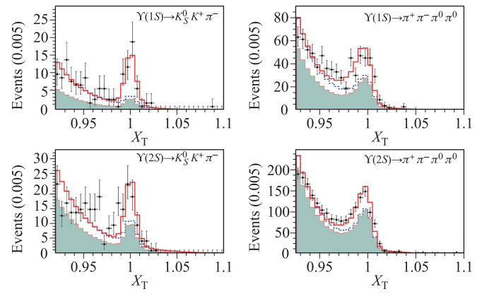
Fig. 3 The fits to the scaled total energy X_T distributions from \Upsilon(1S) and \Upsilon(2S) decays to K_S^0 K^+ \pi^- and \pi^+ \pi^- \pi^0 \pi^0 from Belle [50]. Solid dots with error bars are from resonance data. The open histograms show the best fits, the dashed curves are the total background estimates, and the grey histograms are the normalized continuum background contributions.
