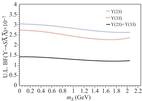
Fig. 15 The 90% C.L. upper limits on the \Upsilon(2S, 3S) \rightarrow S\bar{L}\bar{L} branching fractions for the \Upsilon(2S) and \Upsilon(3S) datasets, as well as the combined sample assuming the same partial width from BaBar [135].
