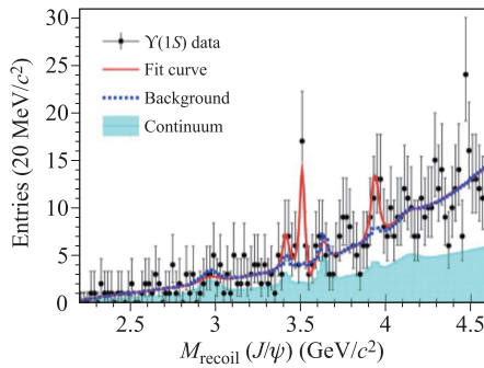
Fig. 6 The recoil mass spectrum against J/\psi in \Upsilon(1S) decays from Belle [72]. The red solid curve is the nominal fit and the blue-dashed curve shows the total background. The fitted normalized continuum contribution is represented by the cyan-shaded histogram.
