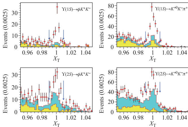
Fig. 2 Scaled total energy, X_T , distributions from \Upsilon(1S) and \Upsilon(2S) decays to \phi K^+ K^- and K^*(892)^0 K^- \pi^+ from Belle [49]. The red dots with error bars are from resonance data, the yellow-shaded histograms are from the normalized continuum contributions described in the text, and the cyan-shaded histograms are from the normalized inclusive \Upsilon(1S) and \Upsilon(2S) MC events. The blue arrows show the required signal regions.
