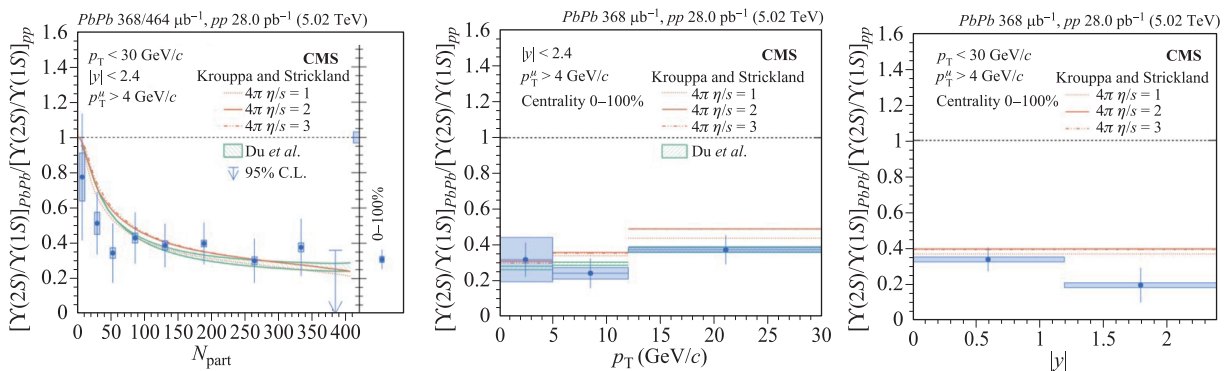
Fig. 33 The double ratios for \Upsilon(2S) as a function of the collision centrality, transverse momentum, and rapidity from CMS [222].
