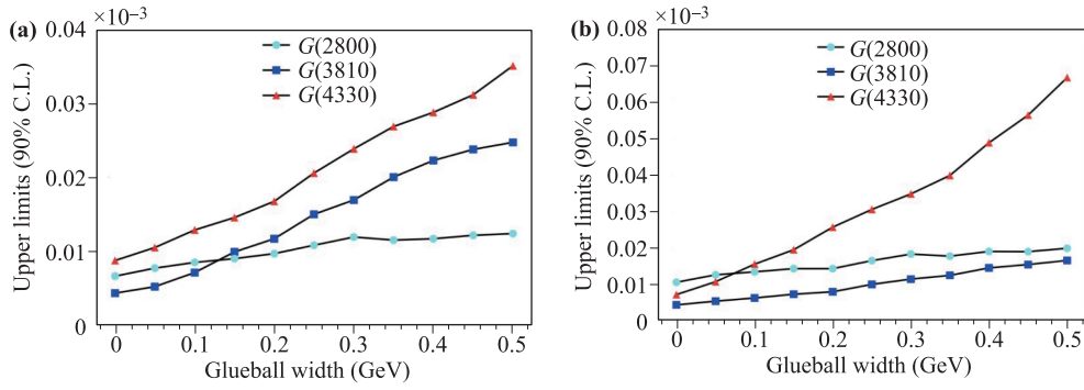
Fig. 13 The upper limits on the branching fractions for (a) \Upsilon(1S) \rightarrow \chi_{c1} + G_{0--} and (b) \Upsilon(2S) \rightarrow \chi_{c1} + G_{0--} as a function of the assumed G_{0--} decay width from Belle [58].
