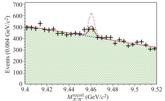
Fig. 16 Recoil mass distribution against two pions, M_{\pi^+\pi^-}^{\text{recoil}} , from Belle [136]. The solid curve shows the result of the fit to the data, the shaded area shows the total background contribution, the dashed line shows the combinatorial background contribution, and the dot-dashed line shows the expected signal for \mathcal{B}(\Upsilon(1S) \rightarrow \chi\chi) = 6.0 \times 10^{-3} [22].
