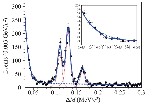
Fig. 12 The distributions of \Delta M in \Upsilon(2S) data from Belle [110]. Dots with error bars are the data, the blue solid curve is the result of the fit for the signal-plus-background hypothesis, and blue dashed curve is background component, respectively. The three \chi_{bJ}(1P) components indicated by the red dotted curves are here considered as part of the signal. The inset shows an expanded view of the \Delta M distribution in the region of [0.035, 0.065] \text{ GeV}/c^2 .
