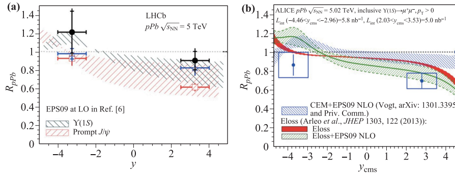
Fig. 38 (a) The nuclear modification factors for \Upsilon(1S) (black dots), prompt J/\psi (red squares), and J/\psi from b -hadron decays (blue triangles) in pPb collisions at \sqrt{s} = 5.02 TeV as a function of rapidity from LHCb [236]. (b) The nuclear modification factors for \Upsilon(1S) in pPb collisions at \sqrt{s} = 5.02 TeV as a function of rapidity from ALICE [237].
