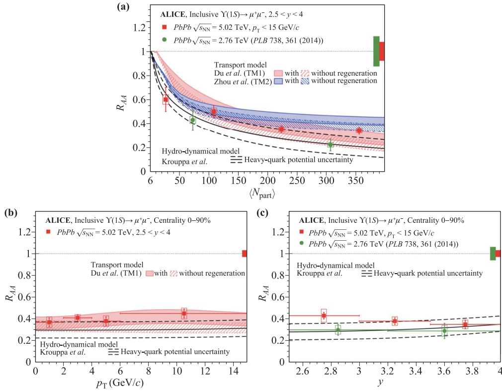
Fig. 34 The R_{AA} factor of \Upsilon(1S) as a function of centrality (a), p_T (b) and y (c) at \sqrt{s} = 2.76 TeV [183] and \sqrt{s} = 5.02 TeV [225] from ALICE.
