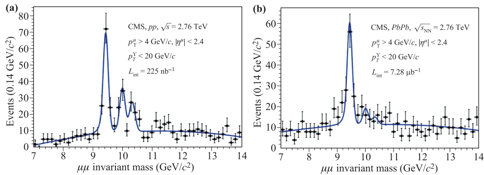
Fig. 30 Dimuon invariant mass distributions obtained with the (a) 225 \text{ nb}^{-1} pp and (b) 7.28 \mu\text{b}^{-1} PbPb data samples at \sqrt{s} = 2.76 TeV from CMS [219]. The solid lines show the best fits to the data.
