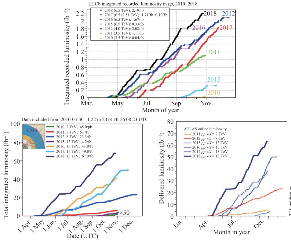
Fig. 22 The integrated luminosities of the pp data recorded by LHCb, CMS, and ATLAS in the past decade [173].
