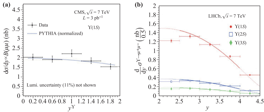
Fig. 24 The differential \Upsilon cross sections as a function of rapidity y varying from 0.0 to 2.0 from CMS [180] (a) and 2.0 to 4.5 from LHCb [186] (b) in the transverse momentum range of p_T < 30 GeV/c. In the left plot, the blue dashed line shows the normalized PYTHIA prediction [185]. In the right plot, the thick lines show the fit results with NRQCD color-octet model predictions from Refs. [187, 188] in the region 2.0 < y < 4.0 , and dashed lines show the extrapolations to the full region 2.0 < y < 4.5 .
