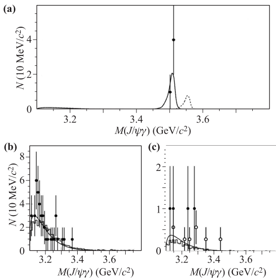
Fig. 8 The J/\psi\gamma invariant mass spectrum in the \Upsilon(1S) data from Belle [76]: (a) M_{\text{rec}} (the mass recoiling against a pion pair) signal window, (b) 20 times wider J/\psi mass sidebands, (c) 20 times wider M_{\text{rec}} mass sidebands. Histograms are the background expectation from the MC simulation from: (b) \Upsilon(1S) \rightarrow \gamma_{\text{FSR}}\mu^+\mu^- , (c) e^+e^- \rightarrow \gamma_{\text{ISR}}\psi' . The solid lines show the result of the simultaneous fit to all these distributions. The dotted line in (a) shows the upper limit on the \chi_{c2} signal yield at 90% C.L.
