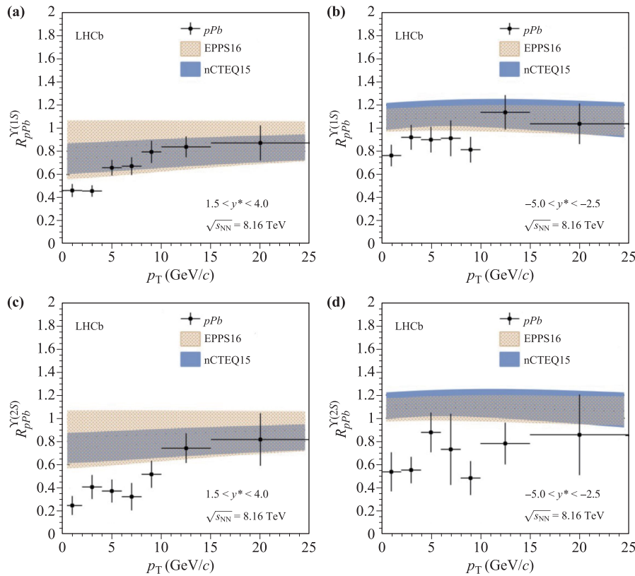
Fig. 39 The nuclear modification factors for \Upsilon(1S) (above) and \Upsilon(2S) (below) in pPb collisions as a function of p_T in the forward (left) and backward (right) regions from LHCb [242].
