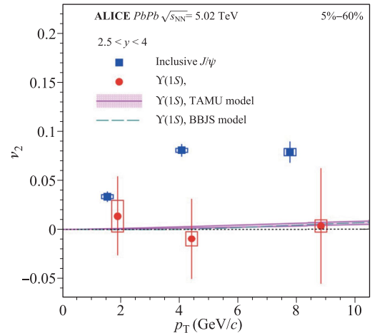
Fig. 36 The \nu_2 coefficient of \Upsilon(1S) as a function of transverse momentum in the rapidity region of 2.5 < y < 4 , compared to that of inclusive J/\psi from ALICE [229].
