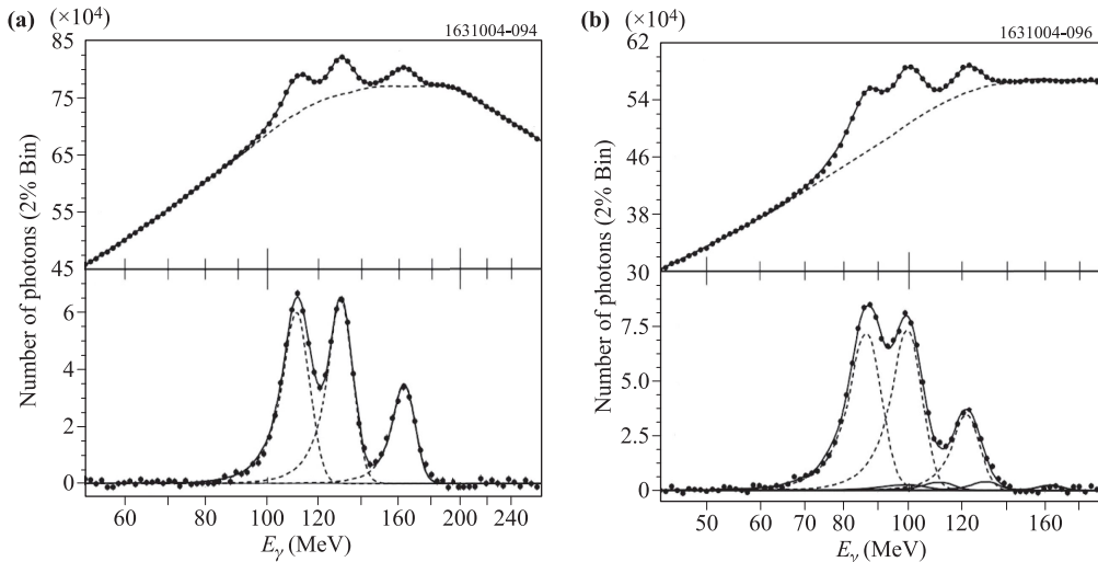
Fig. 9 The energy spectra of photons in (a) \Upsilon(2S) and (b) \Upsilon(3S) decays from CLEO [86]. The dots represent the data (top plot) or the data after subtracting the backgrounds (bottom plot).
