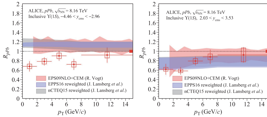
Fig. 40 The nuclear modification factors for \Upsilon(1S) in pPb collisions as a function of p_T in the backward (left) and forward (right) regions from ALICE [243].
