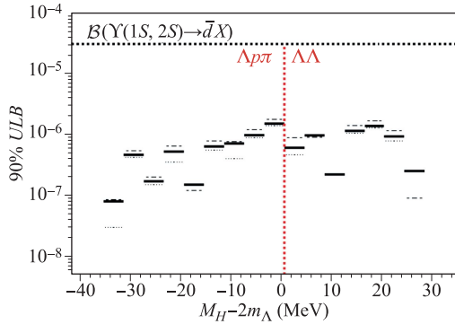
Fig. 14 Upper limits at 90% C.L. for \mathcal{B}(\Upsilon(1S, 2S) \rightarrow H + \text{anything}) for a narrow ( \Gamma = 0 ) H dibaryon versus M_H - 2m_\Lambda are shown as solid horizontal bars from Belle [133]. The +1\sigma ( +2\sigma ) values from the fitted signal yields are shown as the dotted (dashed) bars. (For some mass bins, these are negative and not shown.) The vertical dotted line indicates the M_H = 2m_\Lambda threshold. The horizontal dotted line indicates the average PDG value for \mathcal{B}(\Upsilon(1S, 2S) \rightarrow \bar{d} + \text{anything}) .
