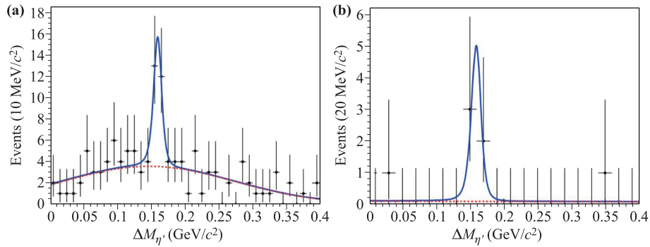
Fig. 20 A simultaneous fit to the \Delta M_{\eta'} distributions for (a) \Upsilon(4S) \rightarrow \Upsilon(1S) + \eta' (\rightarrow \rho^0 \gamma) and (b) \Upsilon(4S) \rightarrow \Upsilon(1S) + \eta' (\rightarrow \eta \pi^+ \pi^-) from Belle [170]. The data, best fit to them, and background contributions are shown by the dots with error bars, solid blue lines, and dashed red lines, respectively.
