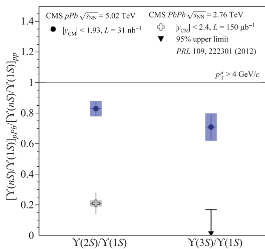
Fig. 37 Event activity integrated double ratios of the excited states, \Upsilon(2S) and \Upsilon(3S) , to the ground state, \Upsilon(1S) , in pPb collisions at \sqrt{s} = 5.02 TeV with respect to pp collisions at \sqrt{s} = 2.76 TeV from CMS [235], compared to their counterparts for PbPb collisions at \sqrt{s} = 2.76 TeV from CMS [220].
