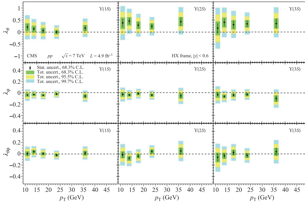
Fig. 28 Values of the \lambda_\theta (top), \lambda_\phi (middle), and \lambda_{\theta\phi} (bottom) parameters for the \Upsilon(1S) (left), \Upsilon(2S) (middle), and \Upsilon(3S) (right) resonances, in the HX frame, as a function of p_T in the rapidity range |y| < 0.6 from CMS [214].
