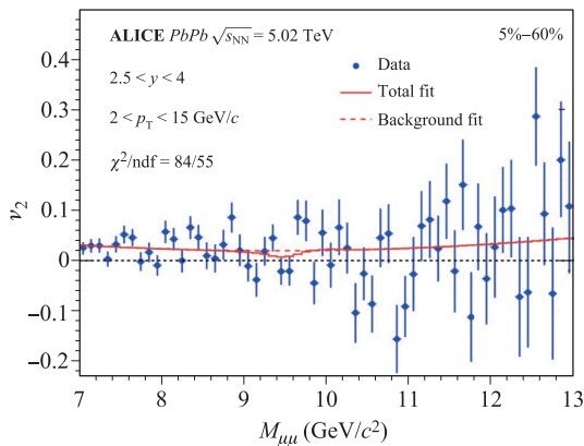
Fig. 35 The graph of \nu_2 with respect to M_{\mu\mu} in the ranges of 2.5 < y < 4 and 2 < p_T < 15 GeV/c from ALICE [229]. The red solid line shows the fitted result, and the red dashed line shows the fitted backgrounds.
