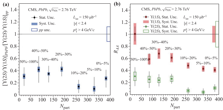
Fig. 32 Centrality dependence of the double ratio (a) and of R_{AA} (b) for the \Upsilon(1S) and \Upsilon(2S) states from CMS [220].
