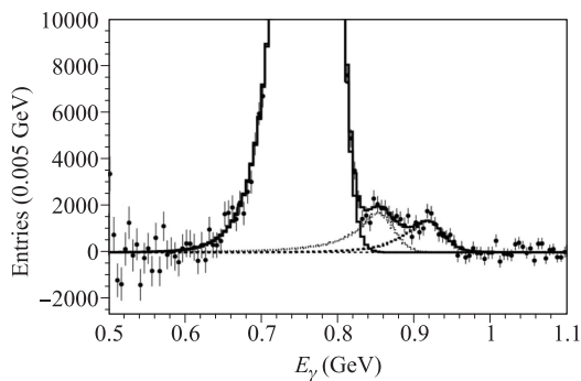
Fig. 10 \Upsilon(3S) inclusive photon spectrum after subtracting the non-peaking background from BaBar [105]. The dots with error bars show the inclusive photon spectrum after subtracting the non-peaking background, and the solid, dotted, and dashed lines show the \chi_{bJ}(2P) peak, ISR \Upsilon(1S) , and \eta_b(1S) signal.
