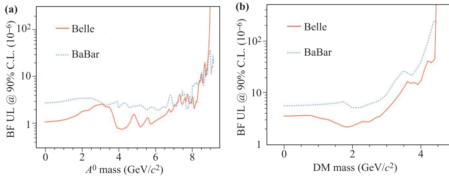
Fig. 18 90% C.L. upper limits on the branching fractions of the on-shell process \Upsilon(1S) \rightarrow \gamma A^0 with A^0 \rightarrow \chi\chi (a) and the off-shell process \Upsilon(1S) \rightarrow \gamma\chi\chi (b). The orange solid curves are the Belle limits [144] and the blue dashed curves are the BaBar limits [145].
