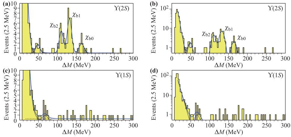
Fig. 11 Distributions of \Delta M \equiv m_{\Upsilon(1S,2S)} - M(\chi_{bb}) in \Upsilon(2S) data (top row) and \Upsilon(1S) data (bottom row) are shown with both linear (left column) and logarithmic (right column) scales using CLEO data [109].
