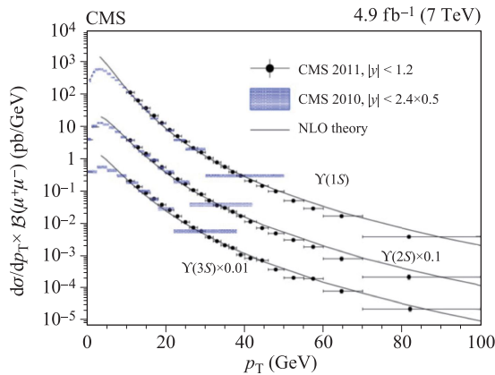
Fig. 26 The differential \Upsilon(1S, 2S, 3S) cross sections times dimuon branching fractions as a function of p_T at \sqrt{s} = 7 \text{ TeV} in the rapidity range of |y| < 1.2 from CMS [201]. The solid lines are the NLO NRQCD color-octet calculations from Ref. [202] extended by the authors to cover the range of p_T < 100 \text{ GeV}/c .
