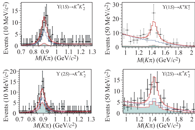
Fig. 1 The invariant mass distributions for K^*(892)^0 candidates and \bar{K}_2^*(1430)^0 candidates from \Upsilon(1S) and \Upsilon(2S) decays from Belle [49]. The open histograms show the results of the two-dimensional fits, the dotted curves show the total background estimates, and the grey histograms are the normalized continuum contributions, which are determined from the data at \sqrt{s} = 10.52 GeV, and extrapolated down to the \Upsilon(1S) and \Upsilon(2S) data.
