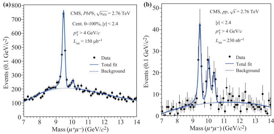
Fig. 31 Dimuon invariant mass distributions from the (a) 150 \mu\text{b}^{-1} PbPb and (b) 230 \text{nb}^{-1} pp data samples at \sqrt{s} = 2.76 TeV from CMS [220]. The solid lines show the best fits to the data, while the dashed lines show the backgrounds.
