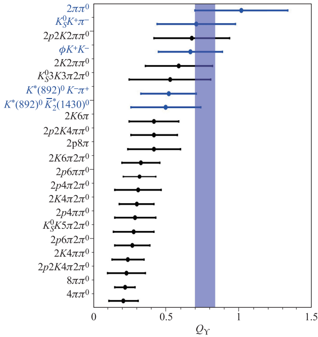
Fig. 4 The Q_Y values for 22 exclusive light hadron decay modes of \Upsilon(1S) and \Upsilon(2S) from Belle [49, 50] (blue dots with error bars) and measurements using CLEO data samples [51] (black dots with error bars). The band shows the theoretical prediction and its uncertainty.
