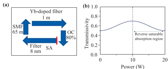
Fig. 55 (a) Schematic of the Yb-doped fiber laser, where SMF indicates single mode fiber, OC is output coupler, and SA means saturable absorber, respectively. Red line is the start and end point for every round trip. (b) Transmissivity as a function of the pump power. Reproduced from Ref. [371].
