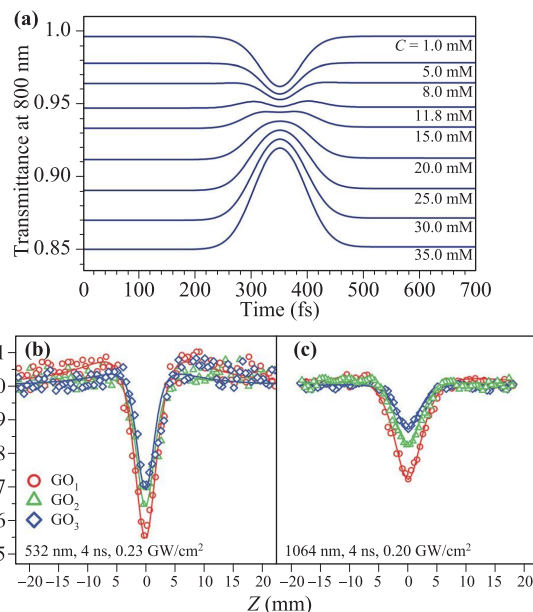
Fig. 56 (a) Variation of transmittance with time for 100 fs pump pulse excitation for different concentration values at a pulse intensity of 5 \times 10^{10} \text{ W}/\text{cm}^2 . Reproduced from Ref. [370]. Open-aperture Z-scans of the GO 1 , GO 2 and GO 3 dispersions under 4 ns at 532 nm (b) and 1064 nm (c) laser excitation. The solid lines correspond to the best fits of the experimental data. Reproduced from Ref. [376].
