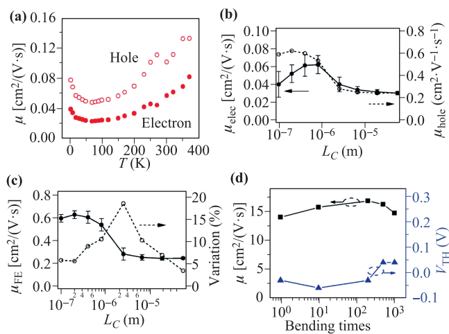
Fig. 39 (a) The electron and hole mobilities ( \mu ) as a function of temperature. Reproduced from Ref. [275]. (b) L_C dependences of field-effect electron ( \mu_{elec} ) and hole ( \mu_{hole} ) mobilities; and (c) L_C dependences of the field-effect hole mobility \mu_{FE} (solid circles) and their variations (open circles). Reproduced from Ref. [279]. (d) Field-effect mobility ( \mu ) and threshold voltage ( V_{TH} ) of the FETs measured after different bending cycle times. Reproduced from Ref. [233].
