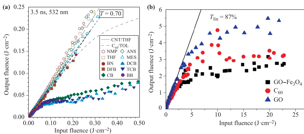
Fig. 59 (a) Plot of output versus input fluence for sub-GO x dispersed in different solvents compared with C_{60} in TOL and single-walled CNT in THF, all in cells with 1.0 mm path length. NMP, N-methylpyrrolidinone; THF, tetrahydrofuran; ANS, anisole; MES, mesitylene; DFB, 1,3-difluorobenzene; BN, benzonitrile; CB, chlorobenzene; BB, bromobenzene; DCB, 1,2-dichlorobenzene; TCB, 1,2,4-trichlorobenzene; TOL, toluene. The linear transmittance T is 0.70. Reproduced from Ref. [375]. (b) Output fluence versus input fluence for GO- Fe_3O_4 , GO and C_{60} with the same linear transmittance of 87% with nanosecond pulses. Reproduced from Ref. [391].
