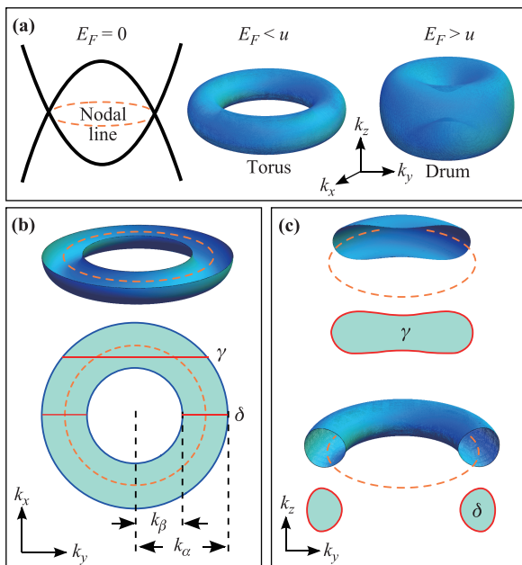
Fig. 3 (a) The nodal line (dashed ring), torus, and drum Fermi surfaces for a generic model of a nodal-line semimetal in Eq. (19). E_F is the Fermi energy. u is a model parameter. (b) The maximum ( \alpha ) and minimum ( \beta ) cross sections in the nodal-line plane of the torus Fermi surface. (c) The maximum ( \gamma ) and minimum ( \delta ) cross sections out of the nodal-line plane of the torus Fermi surface. Reproduced from Ref. [9].
