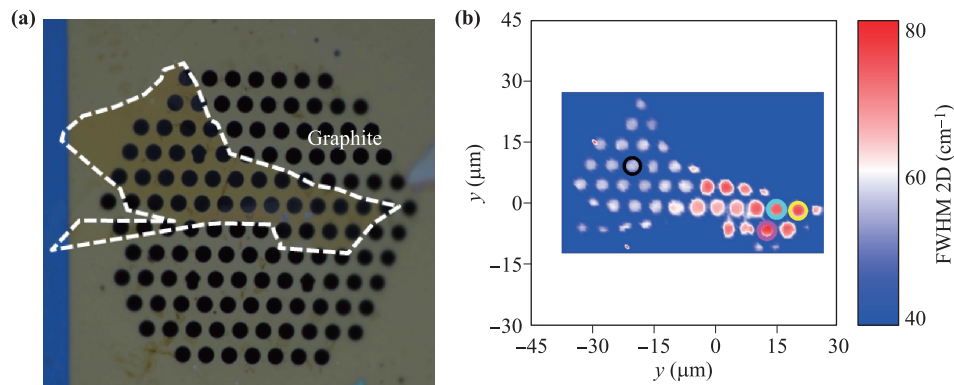
Fig. 3 Raman 2D peak characterization of the few layer graphene (FLG) before transmission electron microscopy (TEM) experiments. (a) Optical micrograph of ABC FLG transferred onto the TEM grid. The white lines correspond to the outline of the graphite flake. (b) The Raman mapping of the 2D peak before the TEM measurements.
