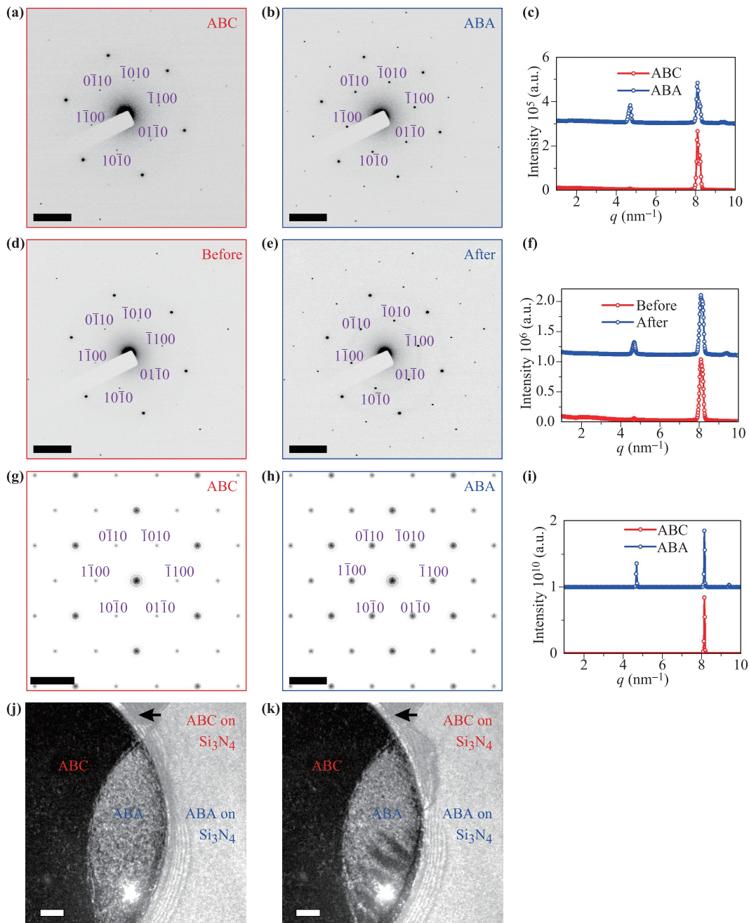
Fig. 4 Electron-diffraction imaging of few layer graphene (FLG). (a, b) Diffraction patterns of ABC FLG [region in the cyan circle in Fig. 3(b)] and ABA FLG [region in the yellow circle in Fig. 3(b)] stacking and the corresponding radial intensity profiles (c). (d, e) Diffraction patterns of ABC FLG [region in the magenta circle in Fig. 3(b)] before and after illuminating the region with train of pulses, showing partial transition from ABC to ABA stacking. (f) Radial intensity distributions of experimental diffraction patterns before and after switching. (g, h) Simulated diffraction patterns of ABC TLG and ABA TLG, and the corresponding patterns radial intensity profiles (i). (j, k) Dark field images of partially switched region [region in the black circle in Fig. 3(b), diffraction peak ( \bar{1}100 ) is selected] before and after illumination with single optical pulses. In (c), (f) and (i), q = k \sin \vartheta , where k = 2\pi/\lambda , \lambda is the wavelength and \vartheta is the scattering angle. The scalebar in (a, b, d, e, g, h) is 5 \text{ nm}^{-1} , and in (j, k) is 200 \text{ nm} .
