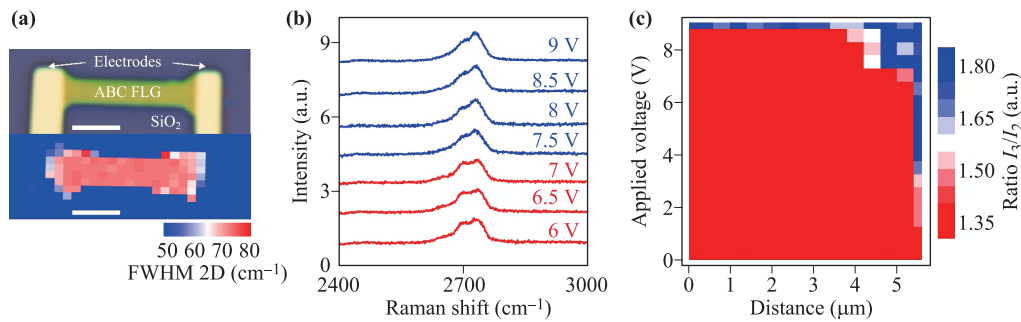
Fig. 2 Raman spectroscopy for the 2D peak characterization of hBN/ABC FLG/hBN device during Joule heating experiment. (a) Top: Optical micrograph of hBN/ABC FLG/hBN device. Bottom: Raman map of full width at half maximum (FWHM) of the 2D peak. Scale bars are 2 \mu\text{m} . (b) Evolution of the Raman spectrum of the 2D peak at 0 V after visiting different bias voltage, measured at distance position 4.8 \mu\text{m} . The blue and red lines indicate the ABA- and ABC-stacking domains, correspondingly. (c) Raman map of I_3/I_2 as a function of distance along the sample and applied voltage, after application of each bias voltage. The red ( R < 1.3 ) and blue ( R > 1.7 ) areas represent the ABC- and ABA-stacking domains, respectively.
