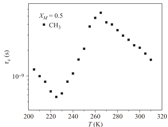
Fig. 4 The rotational correlation time \tau_c as a function of the temperature for methyl groups of methanol at the equimolar composition ( X_M = 0.5 ).
