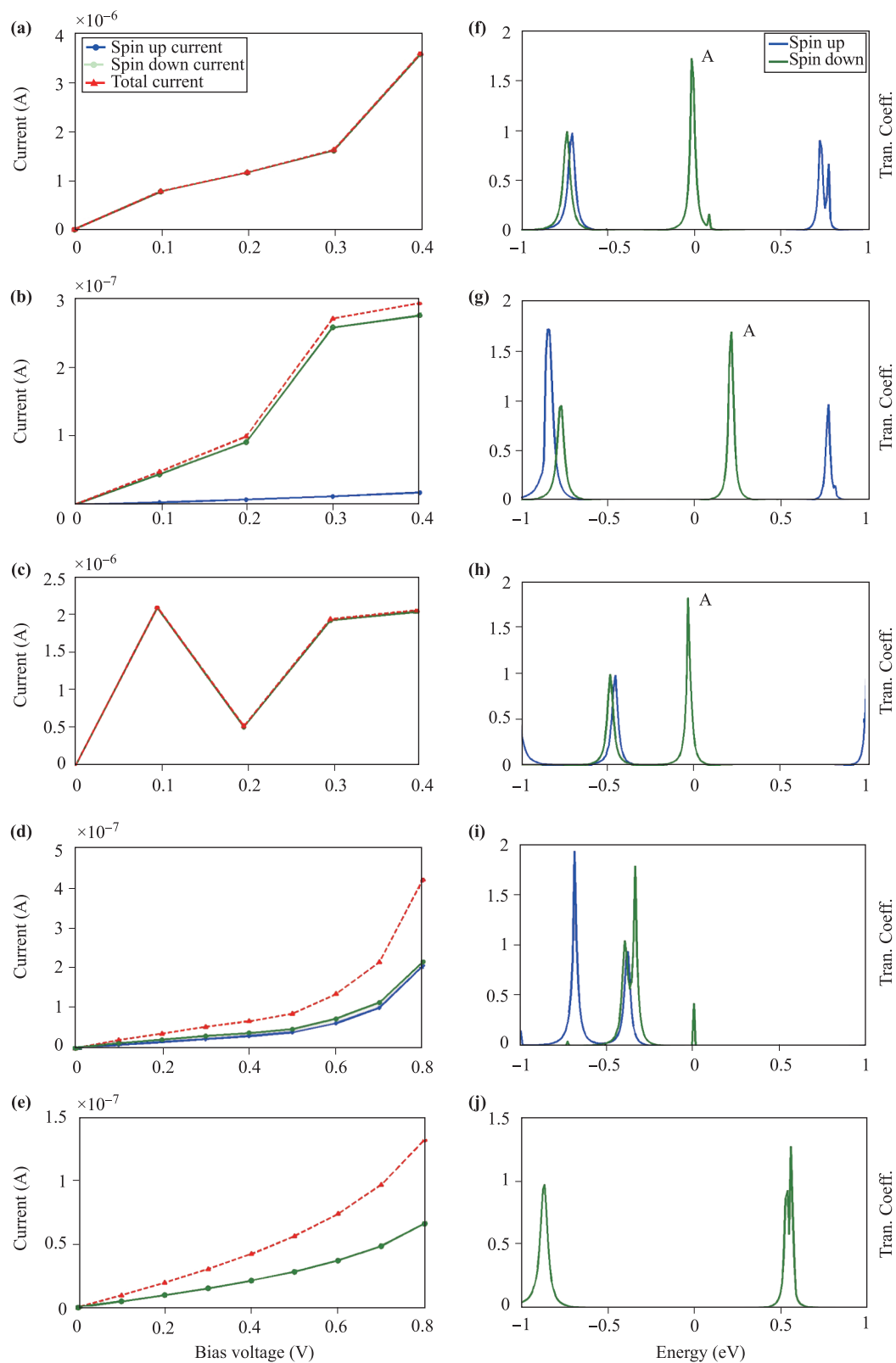
Fig. 2 Current-flowing MPc molecular devices versus bias voltage with different central cations: (a) MnPc; (b) CrPc; (c) FePc; (d) CoPc; (e) NiPc. Transmission coefficient versus energy at zero bias for (f) MnPc; (g) CrPc; (h) FePc; (i) CoPc; (j) NiPc.
