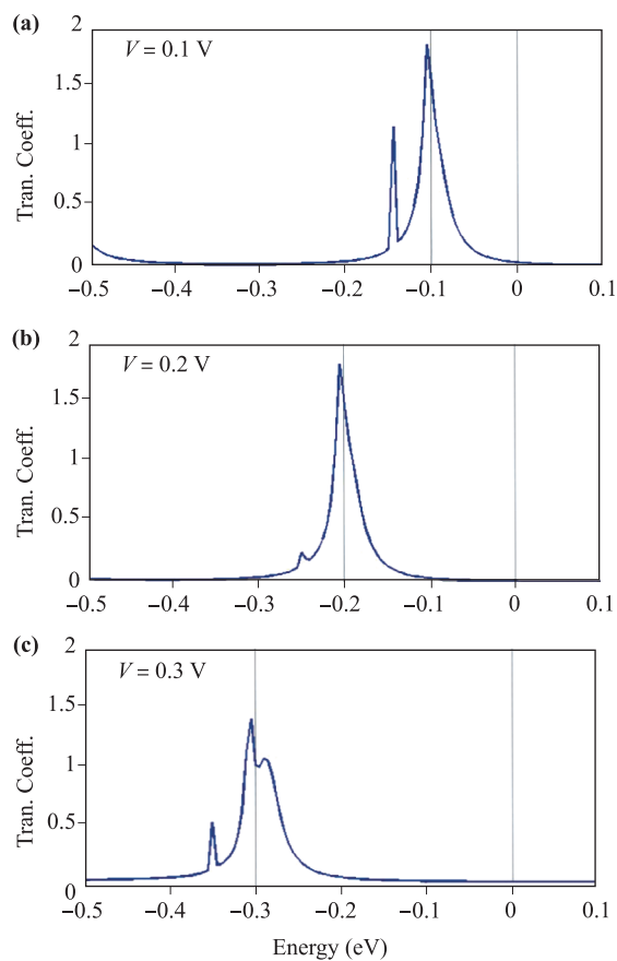
Fig. 4 Transmission coefficient versus energy at different bias voltages.
