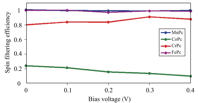
Fig. 3 Spin filtering efficiency at different voltages.
