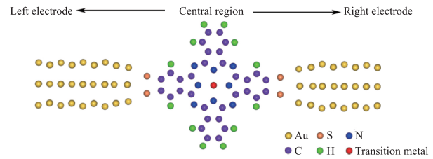
Fig. 1 Schematic plot of the Au(001)-MPc-Au(001) device.
