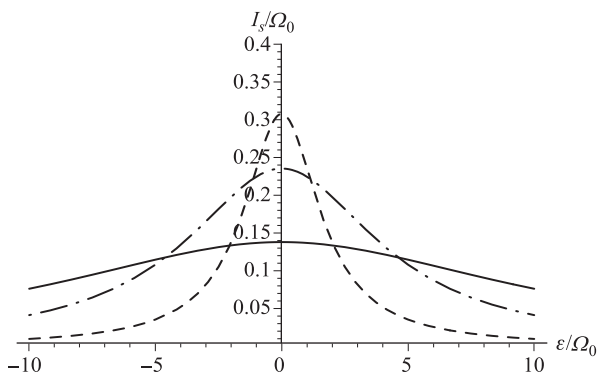
Fig. 13 Electron current through the double-dot, Eq. (126), for \Gamma_L = \Gamma_R = \Omega_0 as a function of the level displacement \epsilon = E_2 - E_1 . The curves correspond to different values of the dephasing rate: \Gamma_d = 0 (dashed), \Gamma_d = 4\Omega_0 (dot-dashed) and \Gamma_d = 16\Omega_0 (solid).
