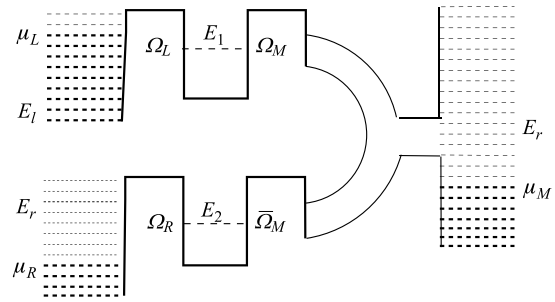
Fig. 7 Two quantum dots, separated by a common reservoir (ballistic channel), as in Fig. 5, where the dots are coupled to the reservoir at spacially close points.
