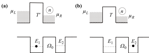
Fig. 10 Electron oscillations in the double-well. The penetration coefficient of the point-contact varies from T' to T when an electron occupies the left well (a) or the right well (b), respectively. The index n denotes the number of electrons accumulated in the collector at time t .
