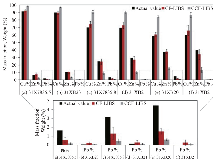
Fig. 4 Results of calculation using the CF-LIBS and CCF-LIBS methods. The subfigure at the bottom shows the enlargement of the Pb mass fraction. Reproduced from Ref. [92], Copyright © 2015 The Authors.
