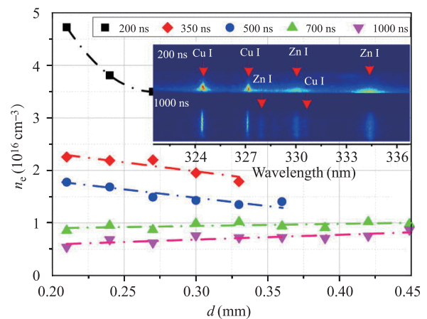
Fig. 2 Electron number density n_e at different distances from the surface of the target with typical spectral images inset. Reproduced from Ref. [25], Copyright © 2013 AIP Publishing LLC.
