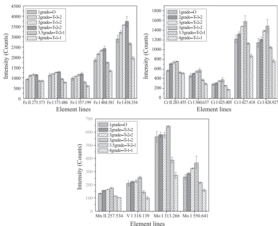
Fig. 6 The peak intensities of the samples. Reproduced from Ref. [123], Copyright © 2015 Elsevier.
