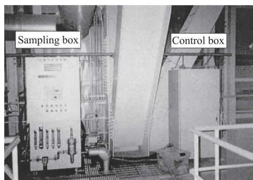
Fig. 9 Photograph of unburned-carbon measurement apparatus. Reproduced from Ref. [177], Copyright © 2003 Optical Society of America.
