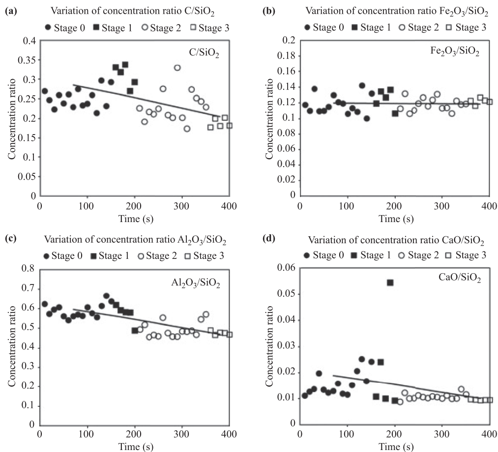
Fig. 5 Real-time LIBS measurement results of fly ash in different stages. Reproduced from Ref. [102], Copyright © 2013 Elsevier.
