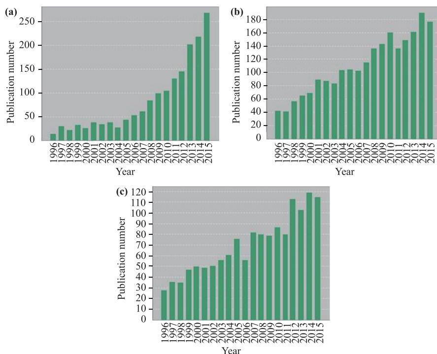
Fig. 1 Statistics of LIBS publications in each year in different territories searched from Web of Science from 1996. (a) Asian countries; (b) European countries; (c) USA and Canada.
