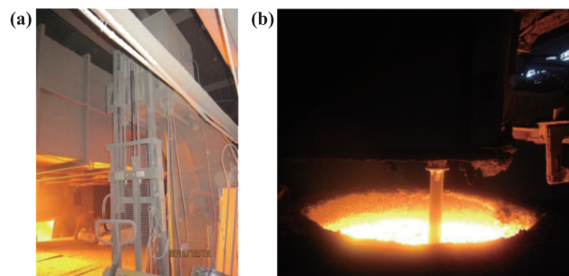
Fig. 8 Application test photos in a steel plant. (a) Sealed LIBS setup installed along the ladle path. (b) The refractory lance tip immersed into the liquid steel in the ladle during measurements. Reproduced from Ref. [176], Copyright © 2015 Elsevier.
