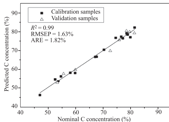
Fig. 3 Calibration and validation results of the combination model of spectrum standardization and dominant factor based PLS method for carbon analysis in coal. Reproduced from Ref. [81], Copyright © 2014 Elsevier.
