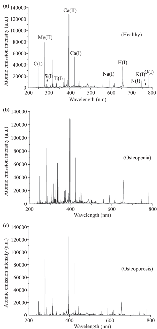
Fig. 7 Characteristic LIBS spectra of human fingernail samples from (a) a healthy with some atomic emissions identified, (b) an osteopenic, and (c) an osteoporotic subject. Reproduced from Ref. [154], Copyright © 2012 AIP Publishing LLC.
