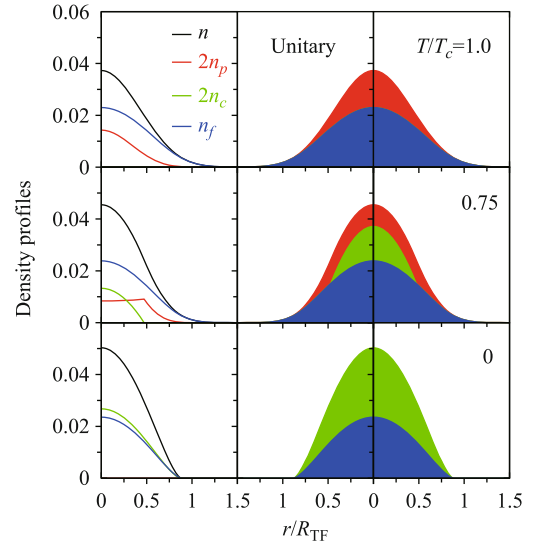
Fig. 17 Decomposition of the density profile n(r) of a Fermi gas in a trap at unitarity for representative temperatures T/T_c = 1, 0.75 , and 0 , as labeled. At T_c , there are only finite momentum pairs (red) and fermions (blue). Below T_c , the condensate (green) develops, and the finite momentum pair contributions decreases. The pair density n_p is nearly uniform inside the superfluid core. At T = 0 , finite momentum pairs disappear and all pairs are condensed.
