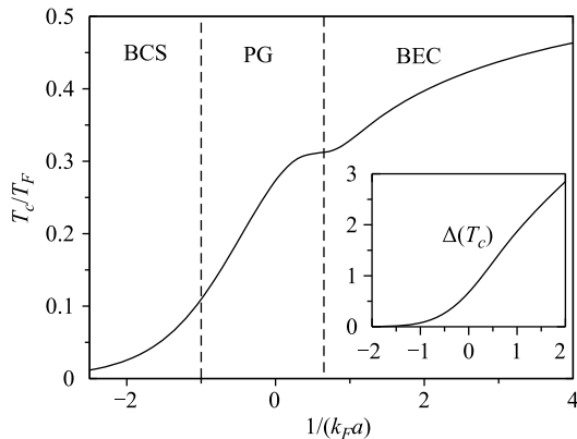
Fig. 15 Behavior of T_c as a function of 1/(k_F a) for a Fermi gas in a 3D isotropic harmonic trap with a short range potential. The plateau is clearly a residue of the maximum–minimum feature in the T_c curve of the homogeneous Fermi gas. As 1/(k_F a) \rightarrow +\infty , T_c approaches its BEC asymptote in a trap, 0.518T_F , where T_F is the global Fermi temperature in the noninteracting limit. The inset shows the behavior of corresponding \Delta(T_c) . Here “PG” denotes pseudogap.
