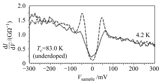
Fig. 5 STM measurements of the dI/dV characteristics of an underdoped Bi2212 sample inside ( solid ) and outside ( dashed ) a vortex core at low T = 4.2 K. Here T_c = 83 K. dI/dV is proportional to the density of states. Reproduced from Ref. [62].
