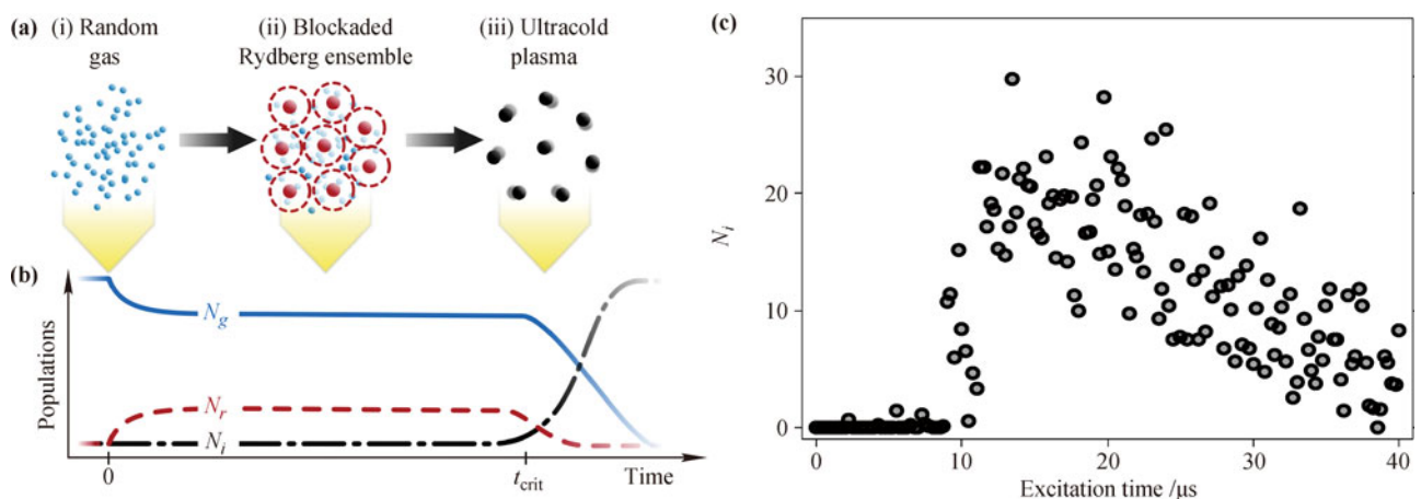
Fig. 10 Generation of an ultracold plasma from a Rydberg-blockaded gas. (a) An initially uncorrelated gas of ultracold atoms is prepared in an optical dipole trap (i). By a doubly resonant two-photon laser excitation some atoms are excited to a Rydberg state. The strong Rydberg–Rydberg interactions prevent the excitation of close-by pairs, leading to spatial correlations (ii). After a time t_{\text{crit}} the Rydberg gas is observed to spontaneously ionize into an ultracold plasma (iii). (b) Qualitative dynamics of the involved populations: ground state atoms N_g (solid line), Rydberg atoms N_r (dashed line), and ions N_i (dash-dotted line). (c) Plasma ion signal taken at a ground state density of \rho = 5 \times 10^{10}\ \text{cm}^{-3} in a volume of \approx 1 \times 10^5\ \mu\text{m}^3 . The rapid ionization avalanche starts after t_{\text{crit}} \approx 10\ \mu\text{s} of continuous excitation.
