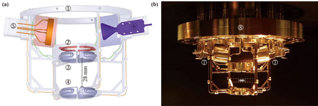
Fig. 6 Electrode assembly for electric field control and for field ionization of Rydberg atoms. (a) Schematic drawing of the electrode assembly for electric field control and for field ionization of Rydberg atoms. A grounded supporting structure ① holds two deflection rings ② as well as four upper ③ and four lower ④ field plates in place, that are used to control the electric field landscape at the position of the atoms. Charged particle detection is possible with either a micro-channel plate detector (MCP) ⑤ or a channel electron multiplier detector (CEM) ⑥. (b) Photograph of the stainless steel structure which also shows the Faraday cages ⑦ that surround the detectors and the vacuum flange ⑧ with 18 high voltage connections. The position of the atom cloud and the orientation of the dipole trap are sketched on the photograph.
