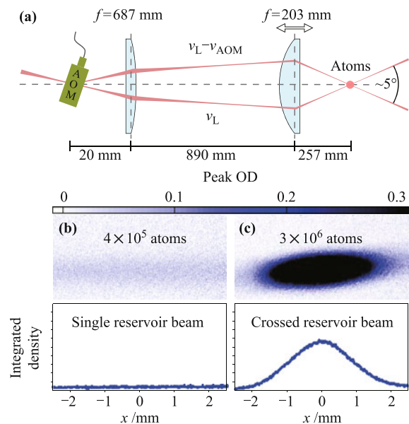
Fig. 3 Atom trapping in a crossed 1064 nm reservoir trap. (a) Schematic of the reservoir trap. An adjustable (double arrow) imaging system with a \approx 0.3 magnification is used to image the diffraction pattern of an acousto-optic modulator (AOM) onto the atom cloud. (b) and (c) show absorption images of a single beam (AOM off) and crossed (AOM on) reservoir trap, respectively after 2 ms of free expansion. The lower panels show the according integrated density distributions. Using the same all over laser beam power (21.5 W) in both scenarios, the crossed beam trap confines almost one order of magnitude more atoms.
