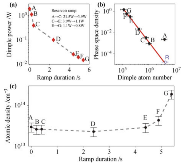
Fig. 4 Optimized evaporative cooling ramp. (a) Adiabatic lowering of the dimple trap power. The evaporative cooling ramp is characterized at the points “A-G”. The inset shows the according reservoir ramp. (b) Inferred phase-space density \varrho_0 versus dimple atom number. The solid line is a power law fit to point “B-G” amounting to a cooling efficiency of \gamma_{\text{evap}} = 3.3 \pm 0.3 . The open square “R” corresponds to the exclusive use of the reservoir trap. (c) shows the evolution of the atomic density (in situ) in the combined trap during the evaporation ramp. The dashed lines serve as guide to the eye.
