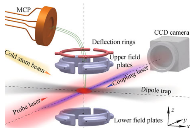
Fig. 1 Experimental system for Rydberg physics in dense ultracold atomic gases. A high flux cold atom beam loads a magneto-optical trap (not shown). The pre-cooled atoms are subsequently transferred into an optical dipole trap, in which evaporative cooling is used for precise temperature and density tuning of the gas. After trap release the atoms are excited to high-lying Rydberg states by a 780 nm probe laser and a counter-propagating 480 nm coupling laser. An electrode structure composed of 8 field plates is used for precise electric field control and for field ionization of Rydberg atoms. Two deflection rings are used to guide the resulting ions (green trajectories) onto a micro-channel plate (MCP) detector. Optical absorption imaging with a CCD camera is done in parallel, providing complementary information.
