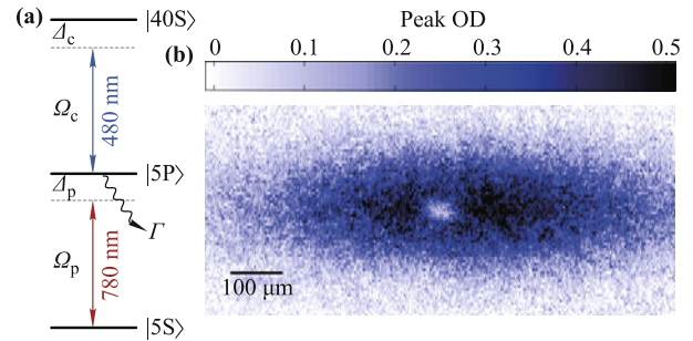
Fig. 8 Optical probing of Rydberg states using electromagnetically induced transparency. (a) Energy level diagram with \Omega_p ( \Omega_c ) the Rabi frequency and \Delta_p ( \Delta_c ) the laser detuning of the 780 nm probe (480 nm coupling) laser, respectively. \Gamma is the spontaneous decay rate of the intermediate |5P\rangle state. (b) Absorption image of the atomic cloud taken after a free expansion of 600 \mu\text{s} , using the laser parameters \Delta_p = \Delta_c = 0 , \Omega_p/(2\pi) = (2.2 \pm 0.3) \text{ MHz} , and \hat{\Omega}_c/(2\pi) = (4.8 \pm 0.2) \text{ MHz} . The induced transparency inside the excitation volume is clearly visible in the center of the absorption image.
