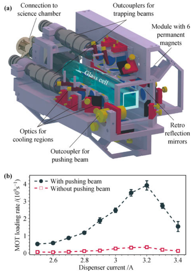
Fig. 2 Technical overview and performance of the 2D-MOT. (a) The UHV glass cell is surrounded by an attachable and externally adjustable, fiber based 2D-MOT cage system. It provides polarization and retro-reflection optics as well as permanent magnets for three cooling regions. (b) Dependence of the loading rate on the ^{87}\text{Rb} dispenser current. The maximum loading rate of (3.9 \pm 0.3) \times 10^9 \text{ s}^{-1} is reached for a current of 3.2 A. We observe a loading rate increase of a factor 12 \pm 2 when operating the 2D-MOT with pushing beam. The dashed lines serve as a guide to the eye.
