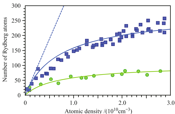
Fig. 9 Measurement of interaction-induced Rydberg excitation suppression. The plot shows the |55S\rangle Rydberg atom number (corrected for the 40% detection efficiency) as a function of the atomic density in the excitation volume. It compares two sets of experiments done with different excitation volumes (see text). The solid lines are fits to the data using the stationary solution of a simple rate equation model. The dashed line indicates the Rydberg atom number for the neglect of interactions.
