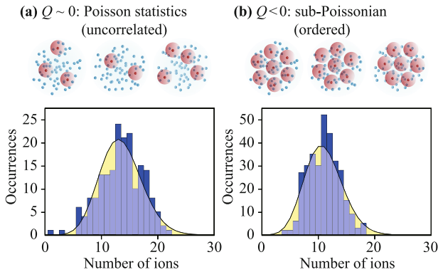
Fig. 11 Counting statistics of Rydberg interacting dark-state polaritons. (a) For low polariton densities we anticipate uncorrelated polariton fluctuations and Poissonian counting statistics with Mandel parameters Q \approx 0 . The lower panel shows counting statistics for 190 consecutive experiments in the low-density regime with \langle N \rangle = 13.5 \pm 0.3 and Q = 0.05^{+0.11}_{-0.10} . (b) Contrary at high densities, we expect a strong suppression of the polariton number fluctuations reflected in sub-Poissonian counting statistics with Q < 0 . The lower panel shows counting statistics for 320 consecutive experiments in the interacting regime yielding \langle N \rangle = 10.99 \pm 0.15 and Q = -0.31^{+0.04}_{-0.05} . The thick curves in both histograms show Poissonian distributions with the corresponding means for comparison.
