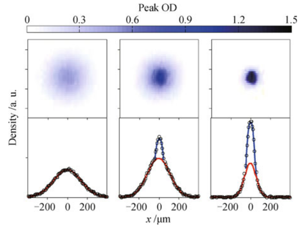
Fig. 5 Bose–Einstein condensation transition. The three columns show measurements for different final beam powers of the dimple trap of 15 mW, 8.4 mW, 2 mW, respectively, taken after a time-of-flight of 22 ms. Upper row: Absorption images of a thermal gas and two partially condensed gases. Lower row: Corresponding integrated atomic density distributions ( points ). The second and third profile clearly show a bimodal structure evidencing the onset of Bose–Einstein condensation. The red lines represent Gaussian fits to the thermal fraction of the gas, whereas the blue lines are Thomas–Fermi profiles quantifying the condensed fraction.
