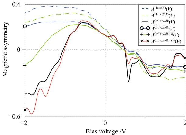
Fig. 12 Comparison of magnetic asymmetries 3.5 \text{ \AA} above a surface Cr atom probed with the flat magnetic tip and the model CrFe tip. A^{\text{Flat},\kappa(E)} , A^{\text{Flat},\kappa(E,V)} , and A^{\text{CrFe},dI/dV} are calculated from the corresponding P and AP spectra shown in Fig. 11. For the CrFe tip we compare the magnetic asymmetry expressions defined in Eqs. (76)–(80). Reproduced from Ref. [10].
