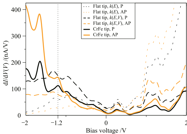
Fig. 11 Comparison of simulated single point differential conductance tunneling spectra following Eq. (41), probed with the flat magnetic tip and the model CrFe tip, 3.5 \text{ \AA} above a surface Cr atom. Parallel (P) and antiparallel (AP) tip magnetization directions are set relative to the underneath surface Cr atom. For the flat magnetic tip, two different vacuum decays, \kappa(E) and \kappa(E, V) are assumed using Eqs. (8) and (15), respectively. The vertical dotted line at -1.2 \text{ V} shows the bias position of the identified STS peak coming from the electronic structure of the CrFe tip. Reproduced from Ref. [10].
