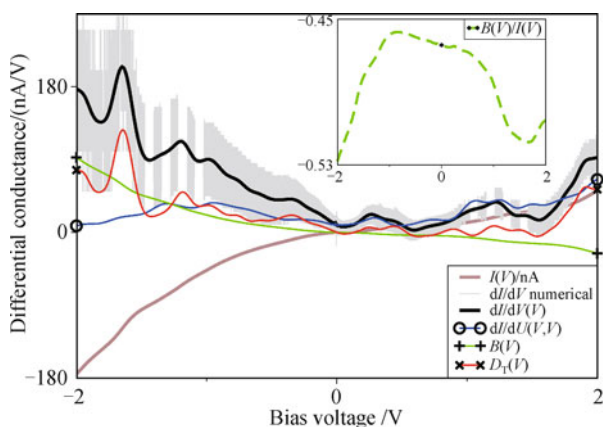
Fig. 10 Comparison of single point differential conductance tunneling spectra calculated from numerical differentiation of the tunneling current I(V) , and dI/dV calculated according to Eq. (41), and its contributing terms, the virtual differential conductance dI/dU(V, V) , the background term B(V) , and the tip-derivative term D_T(V) . The model CrFe tip apex is 3.5 \text{ \AA} above a surface Cr atom and its magnetization direction is parallel to that of the underlying surface Cr atom. The inset shows the ratio of B(V)/I(V) . Reproduced from Ref. [10].
