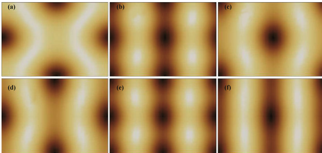
Fig. 18 Comparison of simulated STM images of the W(110) surface using the orbital dependent 3D WKB model with an s -type tip [top, (a)–(c)] and the Tersoff–Hamann model [bottom, (d)–(f)] at V = -0.25 V bias voltage. The scan area corresponds to the rectangle shown in Fig. 14. Light and dark areas denote higher and lower apparent heights, respectively. The apparent heights of the W atom ( z_T ), and the corrugation of the contours ( \Delta z' ) are as follows: Orbital dependent 3D WKB model: (a) z_T = 3.80 Å, \Delta z' = 0.23 pm; (b) corrugation inversion, z_T = 4.15 Å, \Delta z' = 0.10 pm; (c) z_T = 4.35 Å, \Delta z' = 0.12 pm. Tersoff–Hamann model: (d) z_T = 3.80 Å, \Delta z' = 1.63 pm; (e) corrugation inversion, z_T = 4.21 Å, \Delta z' = 1.82 pm; (f) z_T = 4.70 Å, \Delta z' = 1.79 pm. Reproduced from Ref. [91].
