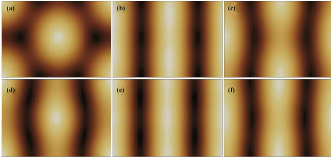
Fig. 19 Comparison of simulated STM images of the W(110) surface using the orbital dependent 3D WKB model [top, (a)–(c)] and the Bardeen method [bottom, (d)–(f)] with the W(110) tip at V = -0.25 V bias voltage. The scan area corresponds to the rectangle shown in Fig. 14. Light and dark areas denote higher and lower apparent heights, respectively. The current values ( I ), the apparent heights of the W atom ( z_T ), and the corrugation of the contours ( \Delta z' ) are as follows: Orbital dependent 3D WKB model: (a) I = 6.3 nA, z_T = 4.50 Å, \Delta z' = 0.36 pm; (b) corrugation inversion, I = 0.43 nA, z_T = 5.80 Å, \Delta z' = 0.02 pm; (c) I = 0.35 nA, z_T = 5.90 Å, \Delta z' = 0.02 pm. Bardeen method: (d) I = 4.4 nA, z_T = 4.50 Å, \Delta z' = 0.07 pm; (e) corrugation inversion, I = 0.7 nA, z_T = 5.55 Å, \Delta z' = 0.03 pm; (f) I = 0.19 nA, z_T = 6.25 Å, \Delta z' = 0.02 pm. Reproduced from Ref. [91].
