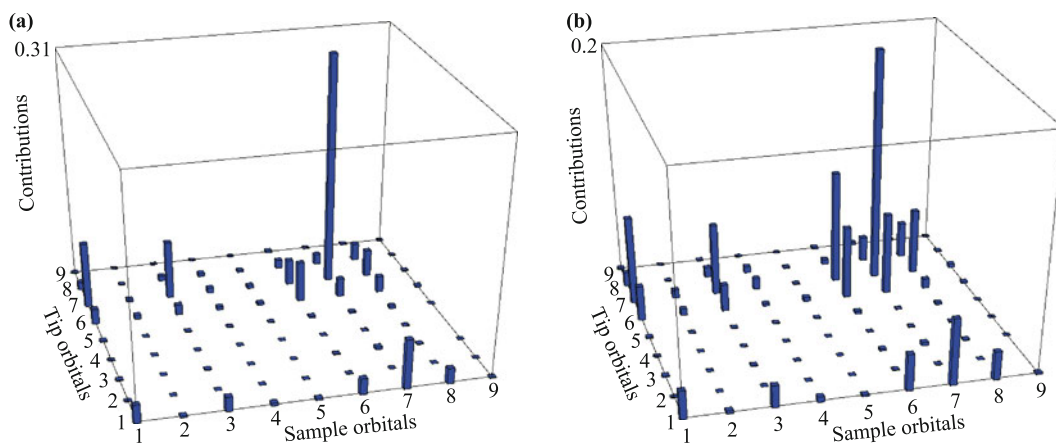
Fig. 16 Histograms of the current contributions ( I_{\beta\gamma} ) from all tip-sample transitions with different orbital symmetries using the W(110) tip at V = -0.1 \text{ V} bias. (a) Tip apex z = 4.5 \text{ \AA} above the surface top (T) position (W atom); (b) tip apex z = 4.5 \text{ \AA} above the surface hollow (H) position, see also Fig. 14. The indices of the atomic orbitals (1–9) follow the notation reported in Table 2. Reproduced from Ref. [91].
