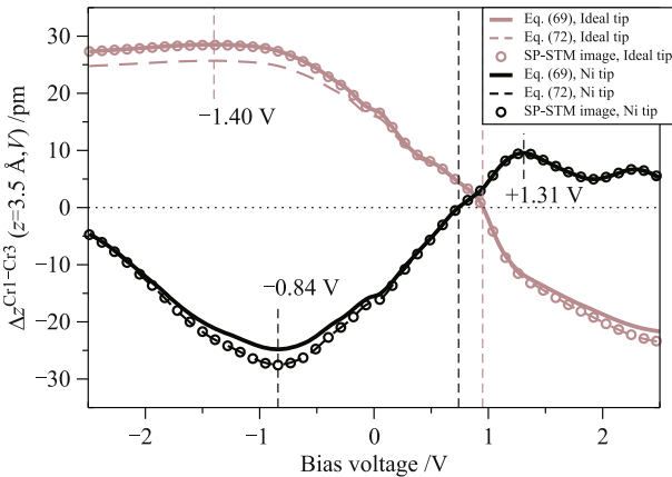
Fig. 6 The bias dependent magnetic contrast between Cr1 and Cr3 atoms \Delta z^{\text{Cr1-Cr3}}(z = 3.5 \text{ \AA}, V) at z = 3.5 \text{ \AA} tip-sample distance calculated using Eq. (69) (solid lines) and Eq. (72) (dashed lines) measured with the ideal magnetic tip (gray) and the Ni tip (black). The tip magnetization direction is fixed parallel to the Cr1 magnetic moment. The local absolute maxima of the magnetic contrasts and their bias values are explicitly shown in both the negative and the positive bias ranges. Vertical dashed lines at 0.74 V and 0.94 V denote the contrast reversals. For comparison, circle symbols show the apparent height difference between Cr1 and Cr3 atoms obtained from constant current SP-STM images, see text for details. Reproduced from Ref. [57].
