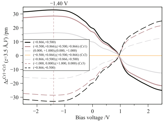
Fig. 9 The effect of the tip magnetization orientation on the bias dependent magnetic contrast between Cr1 and Cr3 atoms \Delta z^{\text{Cr1-Cr3}}(z = 3.5 \text{ \AA}, V) at z = 3.5 Å tip-sample distance calculated using Eq. (69) with the ideal magnetic tip. The unit vectors of the in-plane tip magnetization orientations are rotated in steps of 30^\circ , and are explicitly shown. The parallel or antiparallel orientations with respect to the corresponding Cr magnetic moments are given in parentheses. The absolute contrast maximum of each curve is found at -1.40 V, and is explicitly indicated. Reproduced from Ref. [57].
