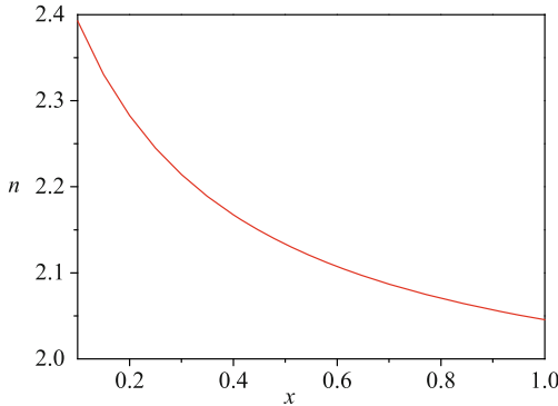
Fig. 14 Refraction index of the composite layer n as a function of the magnitude of the external electric field x is shown. Parameters: p = 0.15 . Reproduced from Ref. [40].
