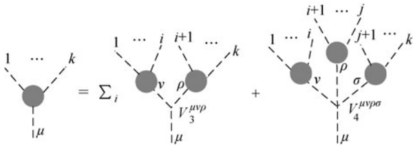
Fig. 3 A graphic description for the off-shell recursion relation of a gluon current.
