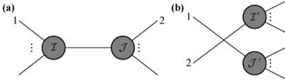
Fig. 4 (a) Diagrams not giving boundary contributions; (b) Diagrams giving boundary contributions.
