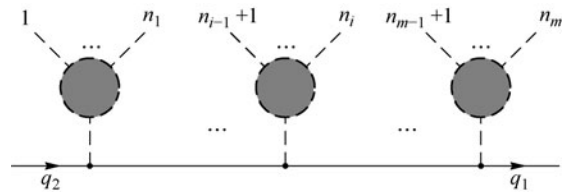
Fig. 5 General Feynman diagrams for the Yukawa theory.
