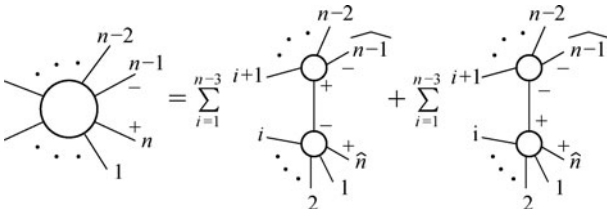
Fig. 1 Pictorial representation of the recursion relation (3.35). Note that the difference between terms in the two sums is the helicity assignment of the internal line.
