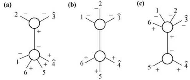
Fig. 2 Configurations contributing to the six-gluon amplitude A_6(1^-, 2^-, 3^-, 4^+, 5^+, 6^+) . Note that (a) and (c) are related by a flip of indices and a complex conjugation, (b) vanishes for either helicity of the internal line.
