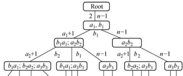
Fig. 8 Graphical representation of tree-level amplitudes of \mathcal{N} = 4 SYM.
