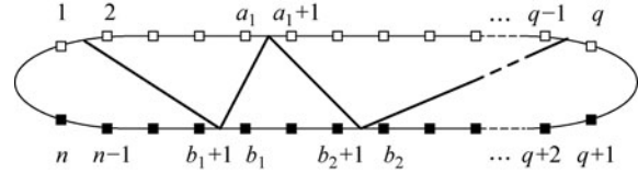
Fig. 6 Zigzag diagrams for split helicity.
