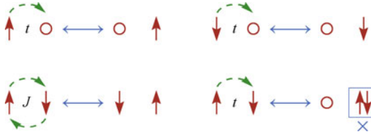
Fig. 4 The first three basic processes are allowed in the t - J model, involving the nearest-neighbor spin-hole states.
