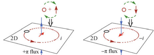
Fig. 8 The phase string effect of the t - J model can be precisely realized via the phase shift factor \Lambda_h in the wavefunction (2).
