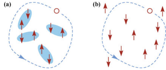
Fig. 12 (a) The motion of the doped hole is coherent in a short-range RVB background; (b) The strongest scattering between the hole and spin degrees of freedom occurs when the background spins are uncorrelated in the high-temperature “strange metal phase”, where each spin carries a fictitious \pm\pi fluxoids as perceived by the hole [cf. also Fig. 6(c)].
