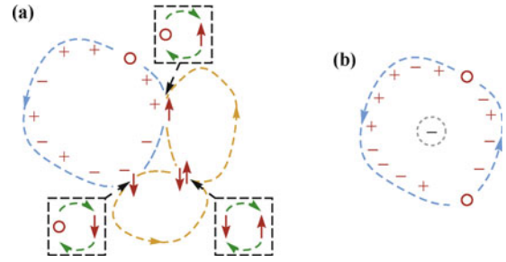
Fig. 5 (a) A phase string associated with a typical closed path of a hole moving on the spin background. Note that the \pm signs are only created by the exchanges between the hole and spins, via \tau_c in Eq. (7), while pure spin loops do not contribute to any signs. (b) The exchange of two holes in a close loop will lead to an additional negative sign to \tau_c .
