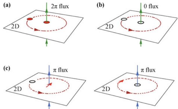
Fig. 9 Statistical transmutations by using the flux attachment based on the boson representation. (a) Fermionic statistics; (b) Bosonic statistics; (c) Mutual semionic statistics.
