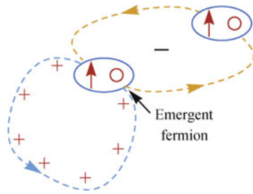
Fig. 7 Coherent fermions may emerge as tightly bound states of hole-spin where a hole hopping always involves the same spin. Note that the bound states are fermionic because of the additional sign upon the exchange of two of them according to Fig. 5(b).
