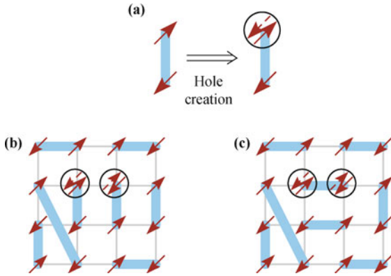
Fig. 2 Schematic illustration of the new superconducting ground state (4). (a) An RVB pair in Fig. 1 becomes a hole-spin pair with the hole (the circle) created by annihilating a spin (as indicated by the dashed arrow), with its RVB partner being automatically associated with the doped hole; (b) and (c) Two doped holes moving on |\text{RVB}\rangle have the tendency to form a Cooper pair as driven by the RVB pairing between their spin partners. Note that the important sign structure of the wavefunction, i.e., \Lambda_h in Eq. (4), is not directly shown here.
