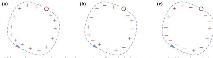
Fig. 6 There will be no frustration from the phase string effect if a hole is moving on the Nagaoka spin background where all the spins are polarized along, say, the \hat{z} -direction as shown in (a). In (b), spins are in the AFM ordered state, where even though the classical Néel order does not lead to the negative total sign, the quantum spin fluctuations can always result in a nontrivial phase string effect as one spin flip can cause the total sign change. One expects the strongest phase string frustration on the coherent motion of the hole if the spins are totally disordered as shown in (c).
