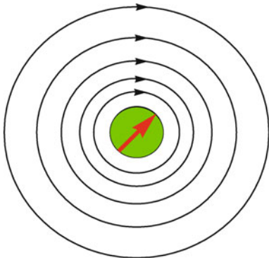
Fig. 11 A spinon-vortex is a composite object with an S = 1/2 free spin locking with a supercurrent vortex. It automatically appears in Eq. (4) if a single spinon is present in |RVB\rangle . A spin-roton excitation in Fig. 10 can be regarded as a vortex-antivortex bound pair of the spinon-vortices.
