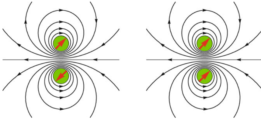
Fig. 10 Spin-rotons with S = 0 and S = 1 , respectively, which are identified [15] as the most essential elementary excitations on top of the ground state (4) and decide the T_c -formula (15).
