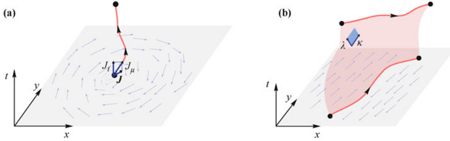
Fig. 2 Vortex world line and world sheet. A graphical picture of dynamical system is provided by tracing the motion of particles or line objects through time. The traces are called world lines or world sheets. In field theory, they are represented by one- or two-form fields, which represent the line or surface elements of the world line or sheet. If the world lines or sheets can not end in the middle of a system, the one- or two-form fields are conserved, as \partial_\mu J_\mu = 0 or \partial_\kappa J_{\kappa\lambda} = 0 . (a) Vortex world line. Segment of a vortex world line (red) in 2+1 dimensions. Shown in blue is the line element J_\mu and its temporal and spatial components J_t and \mathbf{J} . For an electric monopole, these correspond to the charge and current densities \rho and \mathbf{J} . (b) Vortex world sheet. Segment of a vortex line tracing out a world sheet in time. The vortex lies in the x - y -plane, the third spatial dimension cannot be drawn. Shown in blue is the world sheet surface element J_{\kappa\lambda} .
