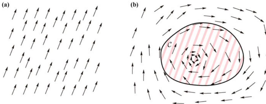
Fig. 1 Phase coherence and its distortion by a vortex. The hallmark of the superconductor is the long-range correlations in the order parameter phase. The phase is a compact variable, and as such permits vortex configurations, that cause the phase to change along its perimeter in multiples of 2\pi only. (a) Phase coherence. Spontaneous symmetry breaking singles out a preferred phase value. (b) Vortex. A single vortex of winding number 1. Tracking the phase change along the contour \mathcal{C} adds up to 2\pi . Also shown in hatched red is the surface \mathcal{S} enclosed by \mathcal{C} .
