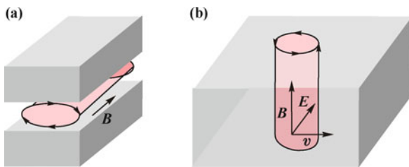
Fig. 3 Additional vortex configurations. (a) A vortex in a Josephson junction between two superconductors (grey); it has no normal core. The magnetic field \mathbf{B} is along the vortex; any electric field across the junction causes the vortex to move in the perpendicular direction. Such motion induces electromagnetic radiation that may escape to the outside world. (b) Vortex. Geometry of the electric field \mathbf{E} generated by a vortex line parallel to the magnetic field \mathbf{B} and moving with a speed \mathbf{v} . This phenomenon related to the Lorentz force follows directly from the vortex equations of motion.
