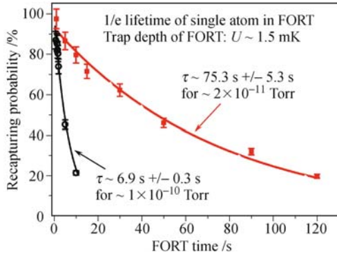
Fig. 7 Trapping lifetime of single atom in the FORT is clearly extended by improving the background pressure. The corresponding solid lines are given by the exponential decay fitting [ P(t) = P_0 \exp(-t/\tau) , \tau is the 1/e trapping lifetime]. The error bars are for \pm 5\% , which is caused partially by imperfect transferring technique and new loading events in transferring process. Each data point is derived from at least 100 sequences.
