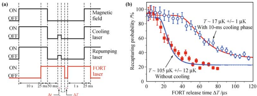
Fig. 6 R&R measurement of a single atom in the FORT. (a) Schematic of the time sequence. \Delta t is the time duration of the laser cooling phase, and \Delta T is the FORT release time. (b) The recapture probability of a single atom as a function of the FORT release time, \Delta T , for the cases with a one-shot 10-ms laser cooling phase (open circles) and without laser cooling (solid squares). The error bars are for \pm 5\% , which is caused partially by imperfect transferring technique and new loading events in transferring process. Each experimental data point is from the accumulation of at least 100 sequences. The solid lines are theoretical fittings according to Eq. (7). The effective temperatures with statistical errors are extracted from the fittings.
