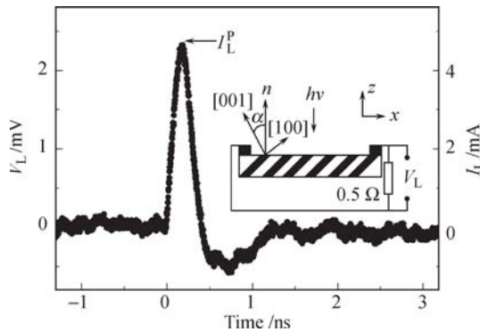
Fig. 1 A typical photovoltage with a 0.5\text{-}\Omega resistance in parallel with the STO single crystal under an excitation of a 25-ps duration and 355-nm laser pulse. The tilted degree \alpha is 15^\circ . The inset displays the schematic circuit of the measurement. I_L^P denotes the peak value of the transient photocurrent.
