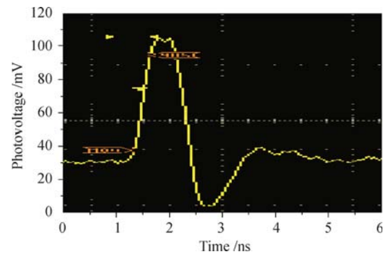
Fig. 3 Variation of the photovoltage with time for LCMO film on tilted 10^\circ STO substrate and a 0.5\text{-}\Omega resistance is connected in parallel with the LCMO film under an excitation using a 25-ps duration and 1.064\text{-nm} laser pulse.
