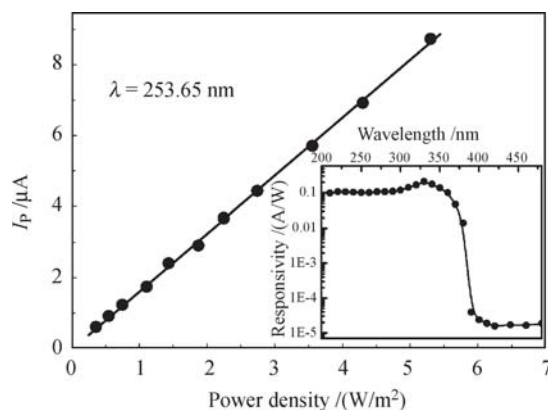
Fig. 9 Photocurrent variation with the power density and the spectral response (inset) of a STO photodetector with 10\text{ }\mu\text{m} finger width and 10\text{ }\mu\text{m} interspacing at 10\text{ V} bias.
