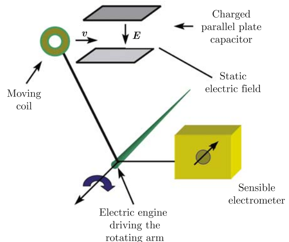
Fig. 2 An example of the untested dual Rowland's experiment. A static electric field E is capable of producing a time-varying magnetic induction in a moving coil. Detection of the induced current or emf in the coil would be an experimental proof of the validity of the dual Rowland's effect.
