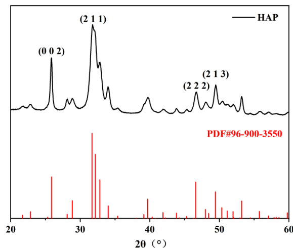
Fig. S1 XRD pattern of nHAP.
