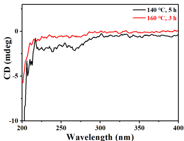
Fig. S1 CD spectra of carbon dots synthesized at 140 °C for 5 h and 160 °C for 3 h.
